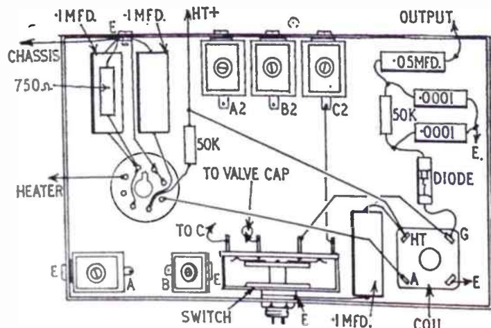
Fig. 2—Wiring diagram of the unit
