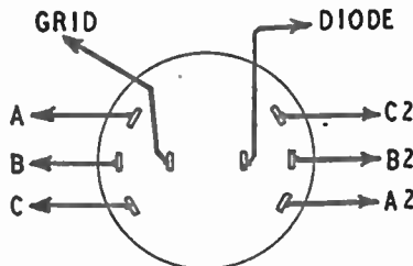
Fig. 3—Connections to the switch
