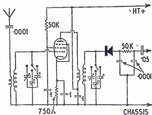
Fig. 1—Tuner circuit
