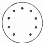
SPECIMEN B9A BASE (Noval)
