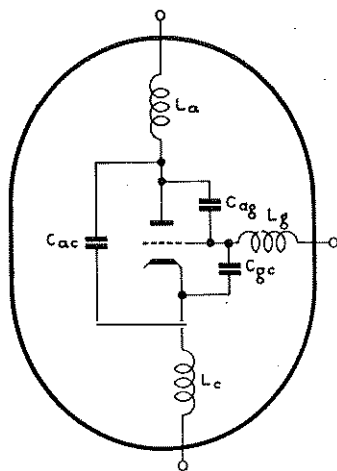
FIG. 1.—SELF-INDUCTANCES AND INTERNAL CAPACITANCES OF A TRIODE VALVE.
