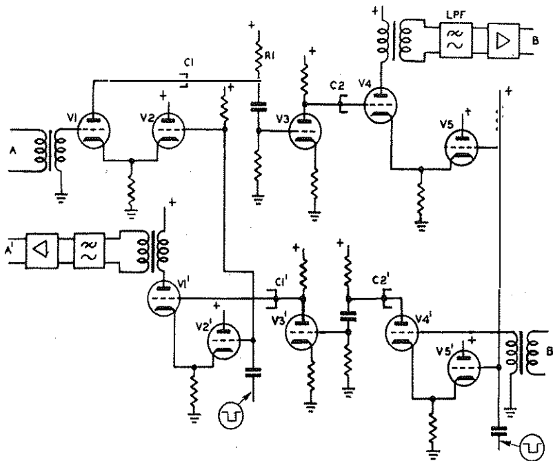
FIG. 11.—SIMPLIFIED CIRCUIT OF AN ELEMENT SWITCH USING PULSE MODULATION TO PROVIDE TWO-WAY COMMUNICATION.
