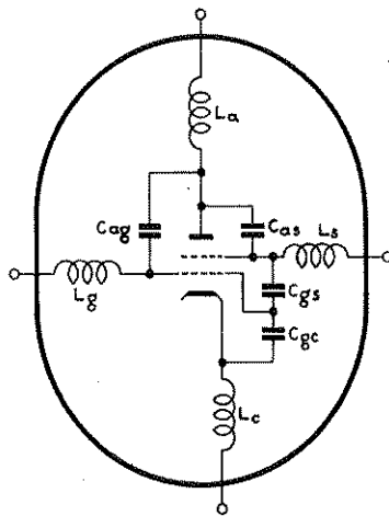
FIG. 2.—SELF-INDUCTANCES AND SOME OF THE MORE IMPORTANT CAPACITANCES OF A TETRODE VALVE.
