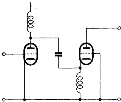
FIG. 6.—SCHEMATIC DIAGRAM OF A "CASCODE" AMPLIFIER.
