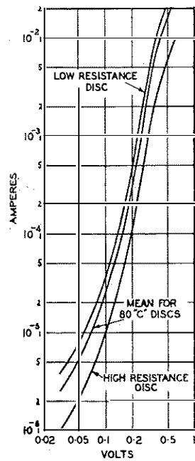
FIG. 7.—TYPICAL RANGE OF CURRENT/VOLTAGE CHARACTERISTICS OF "C" TYPE DISCS.
