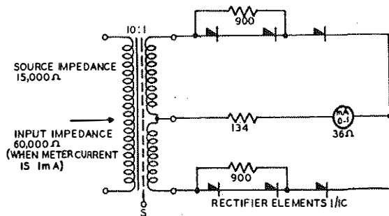
FIG. 4.—RECTIFIER CIRCUIT OF SPEECH VOLTMETER.
