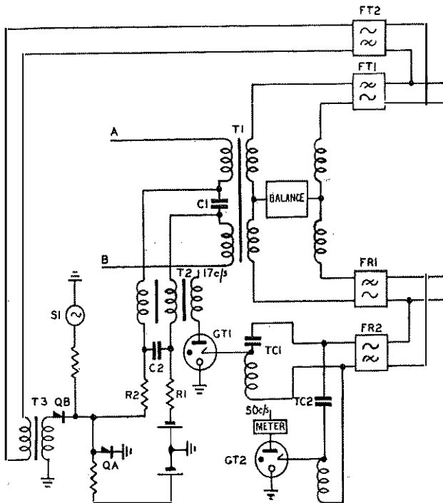
FIG. 13.—A CIRCUIT ARRANGEMENT FOR A SUBSCRIBER'S EQUIPMENT.
