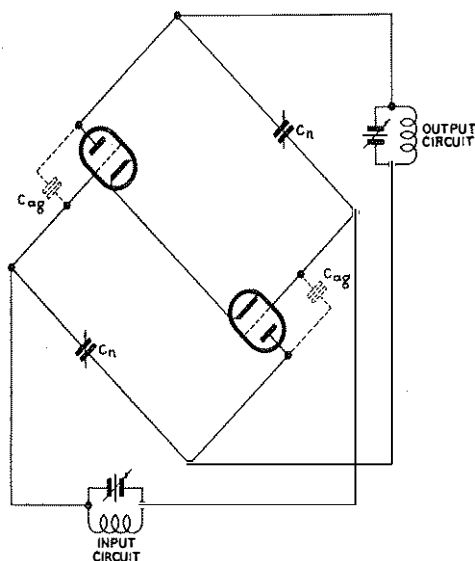
FIG. 3.—TYPICAL NEUTRALISING ARRANGEMENT FOR PUSH-PULL TRIODE AMPLIFIER OPERATING IN BAND 6 OR 7.
