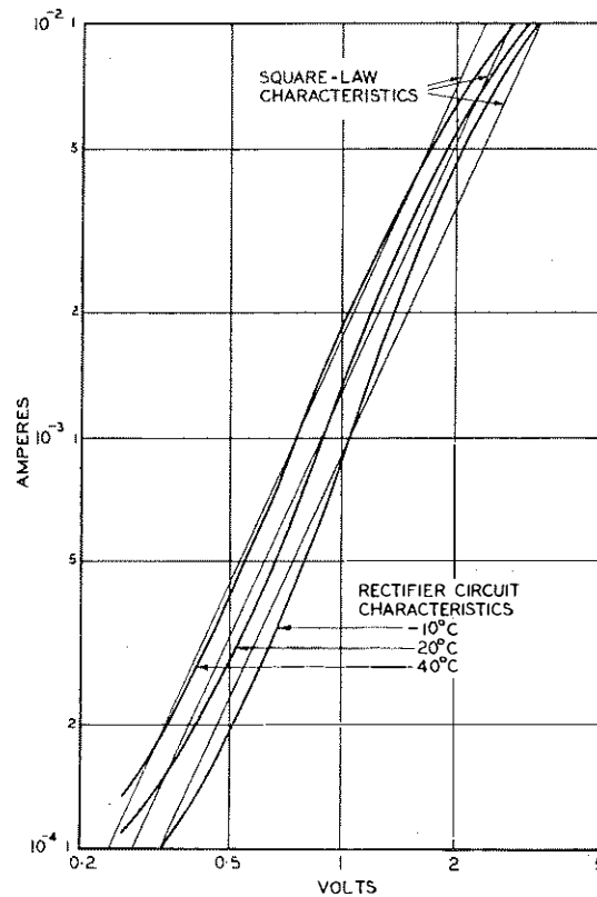
FIG. 9.—EFFECT OF TEMPERATURE VARIATIONS ON CURRENT/E.M.F. CHARACTERISTICS OF RECTIFIER CIRCUIT OF SPEECH VOLTMETER.
