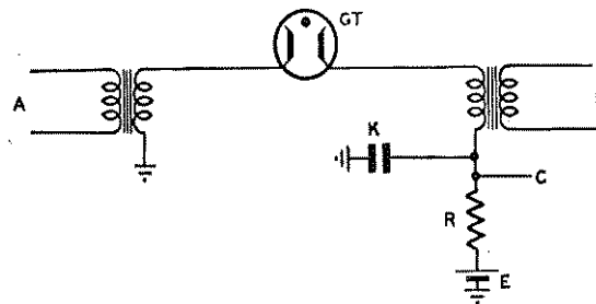
FIG. 6.—ELEMENT SWITCH USING A GAS DISCHARGE TUBE.
