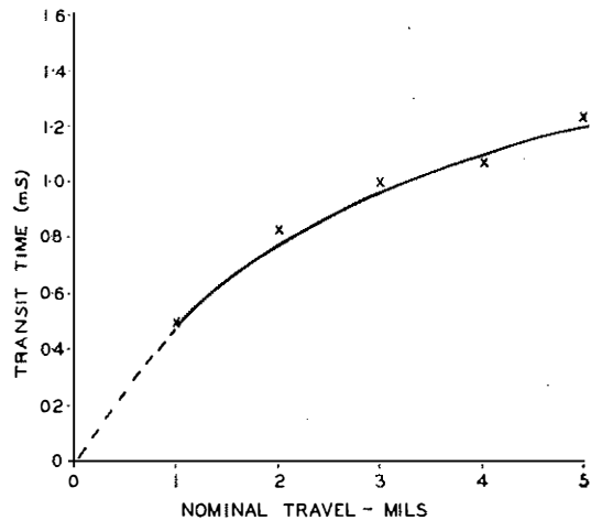
FIG. 8.—RELATION BETWEEN TRANSIT TIME AND TRAVEL WITH ENERGISATION OF 40 AMPERE-TURNS.
