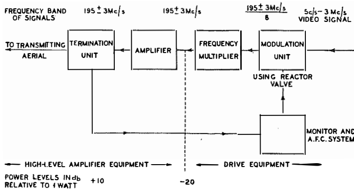
FIG. 10.—SCHEMATIC DIAGRAM OF TERMINAL TRANSMITTER.
