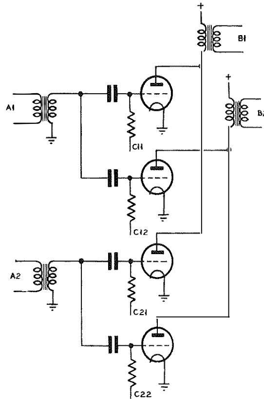
FIG. 5.—A 2.2 SWITCH, USING VACUUM VALVES, BUILT UP FROM 4 ELEMENT SWITCHES.
