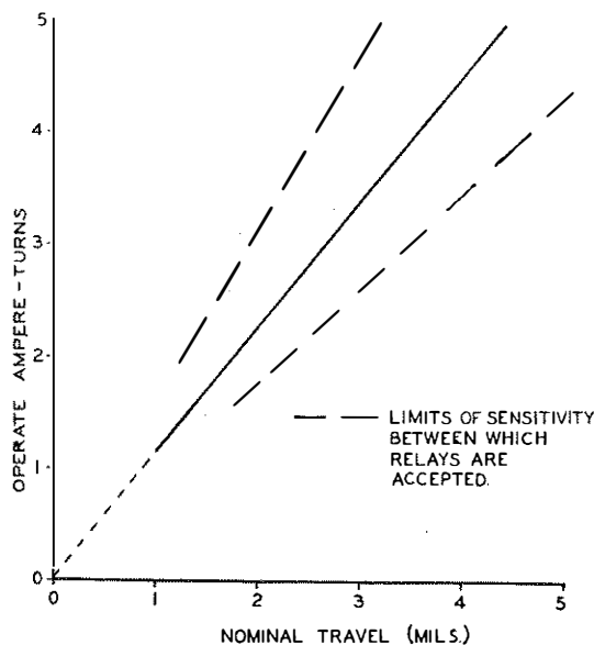
FIG. 7.—RELATION BETWEEN SENSITIVITY AND TRAVEL FOR 7.5 MILS. ARMATURE SUSPENSION SPRING.
