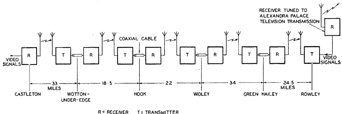
FIG. 4.—SCHEMATIC DIAGRAM OF THE SYSTEM.
