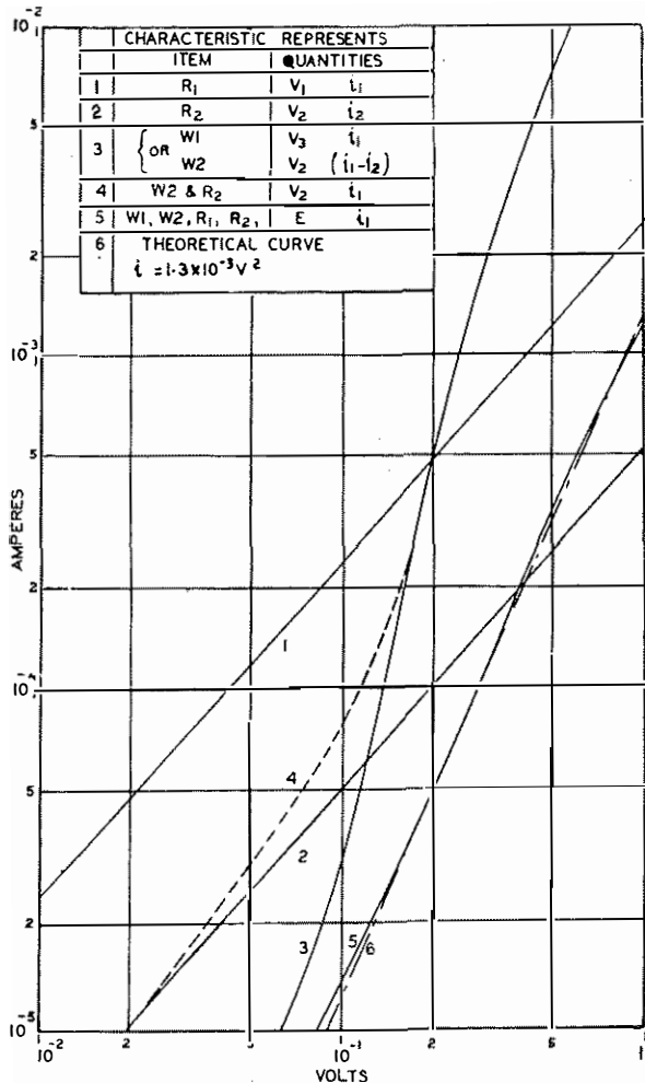
FIG. 2.—GRAPHICAL SYNTHESIS OF BASIC SQUARE-LAW RECTIFIER NETWORK.
