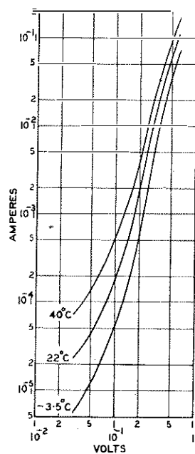
FIG. 8.—EFFECT OF TEMPERATURE VARIATION ON CURRENT/VOLTAGE CHARACTERISTICS OF "C" TYPE DISCS.
