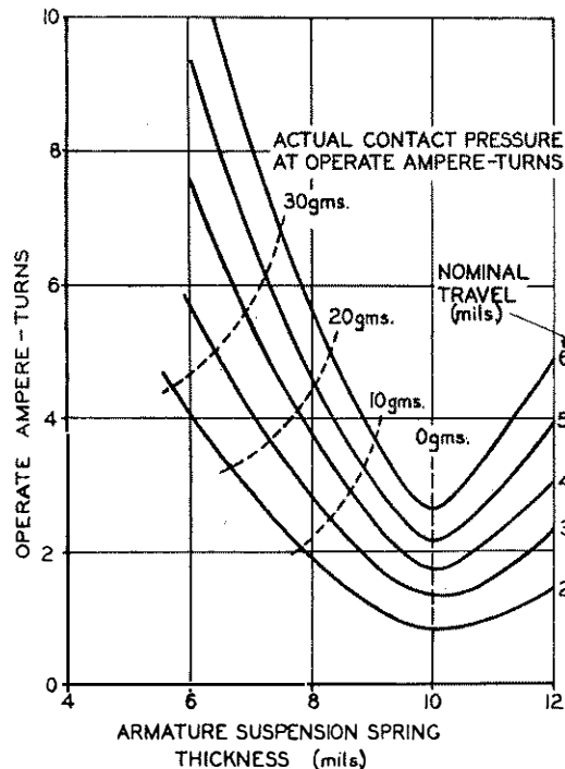
FIG. 6.—RELATION BETWEEN ARMATURE SUSPENSION SPRING THICKNESS AND SENSITIVITY; SHOWING CONTACT PRESSURES AT OPERATE AMPERE-TURNS.
