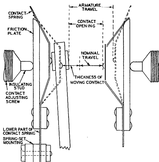
FIG. 5.—THE CONTACT ACTION.
