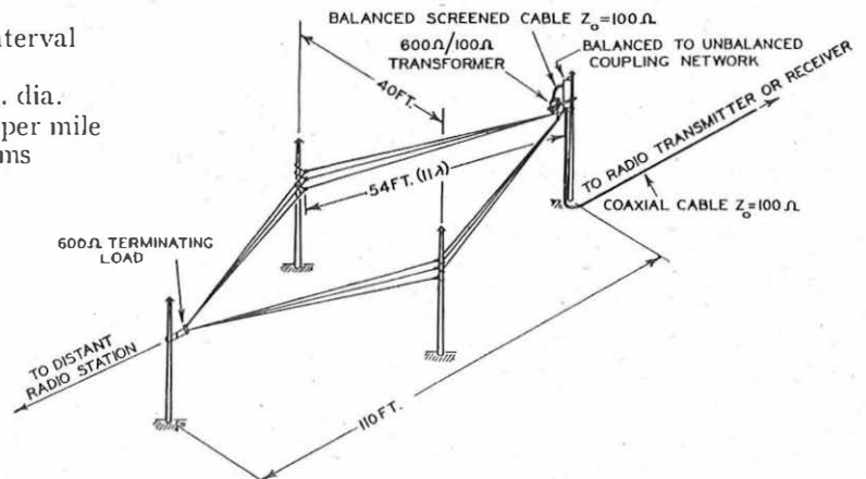
FIG. 9.—TYPICAL ARRANGEMENT OF RHOMBIC AERIAL.
