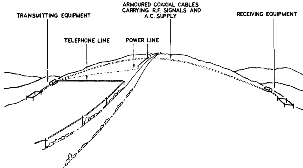
FIG. 3.—LAYOUT OF AN INTERMEDIATE RELAY STATION.
