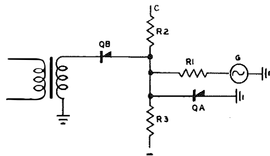
FIG. 12.—A METHOD OF CONTROLLING A.C. FOR SIGNALLING PURPOSES.
