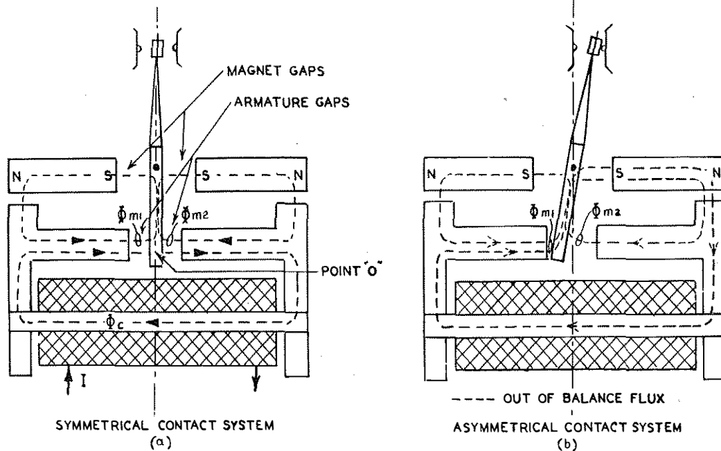
FIG. 3.—THE MAGNETIC CIRCUIT.
