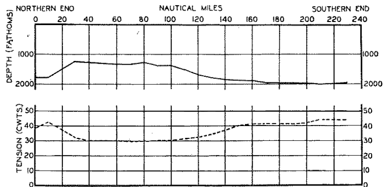
FIG. 5.—GRAPH OF TENSION AND DEPTH FOR MALAGA-LAS PALMAS DIVERSION IN JULY, 1949.
