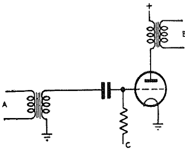
FIG. 4.—ELEMENT SWITCH USING A VACUUM VALVE.
