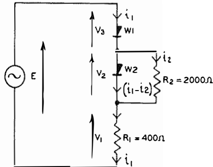
FIG. 1.—BASIC CIRCUIT OF SQUARE-LAW RECTIFIER NETWORK.
