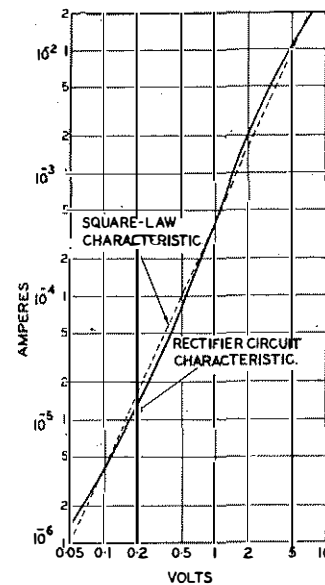
FIG. 6.—CURRENT/E.M.F. CHARACTERISTIC OF RECTIFIER CIRCUIT OF SPEECH ANALYSER.
