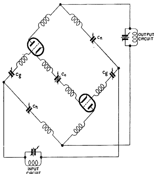
FIG. 4.—TYPICAL NEUTRALISING ARRANGEMENT FOR A PUSH-PULL TRIODE AMPLIFIER OPERATING NEAR TOP OF BAND 8.
