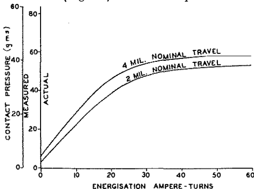
FIG. 10.—RELATION BETWEEN CONTACT PRESSURE AND ENERGISATION.
