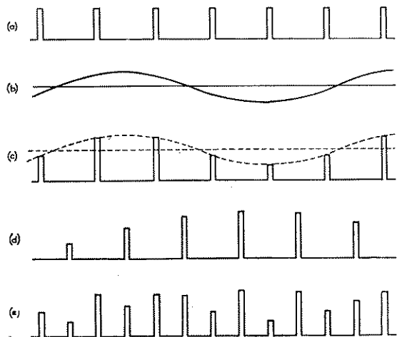
FIG. 10.—GRAPHS ILLUSTRATING THE PRINCIPLE OF TIME-DIVISION-MULTIPLEX TRANSMISSION.
