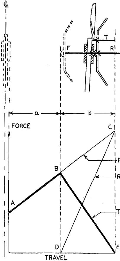
FIG. 9.—MEASUREMENT OF CONTACT PRESSURE WITH A TENSION GAUGE.
