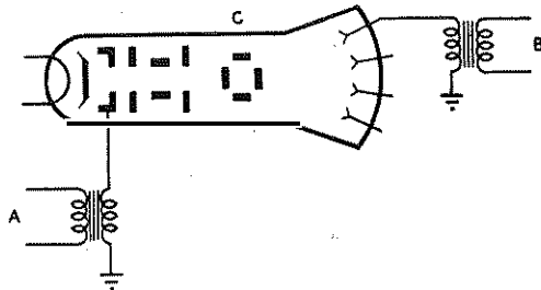
FIG. 8.—ELEMENT SWITCH USING A CATHODE-RAY TUBE.
