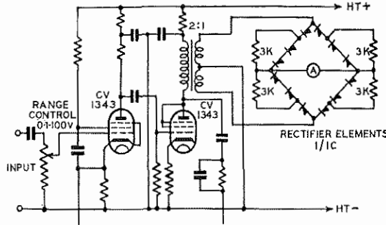
Fig. 3.—AMPLIFIER AND RECTIFIER CIRCUIT OF PSOPHOMETER.
