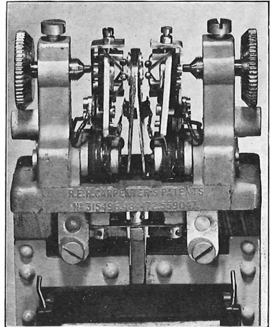
FIG. 11.—CONTACT SYSTEM ON TWO-CHANGEOVER-CONTACT RELAY.
