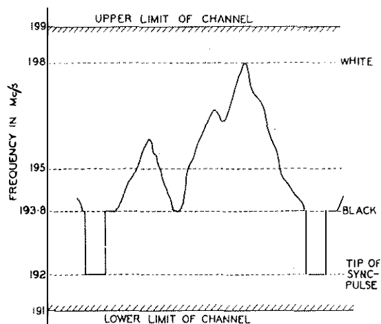
FIG. 2.—THE TRANSMITTED WAVE FORM.
