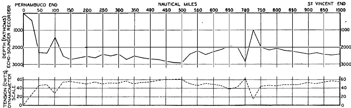
FIG. 4.—GRAPH OF TENSION AND DEPTH FOR ST. VINCENT-PERNAMBUCO RENEWAL IN AUGUST, 1948.
