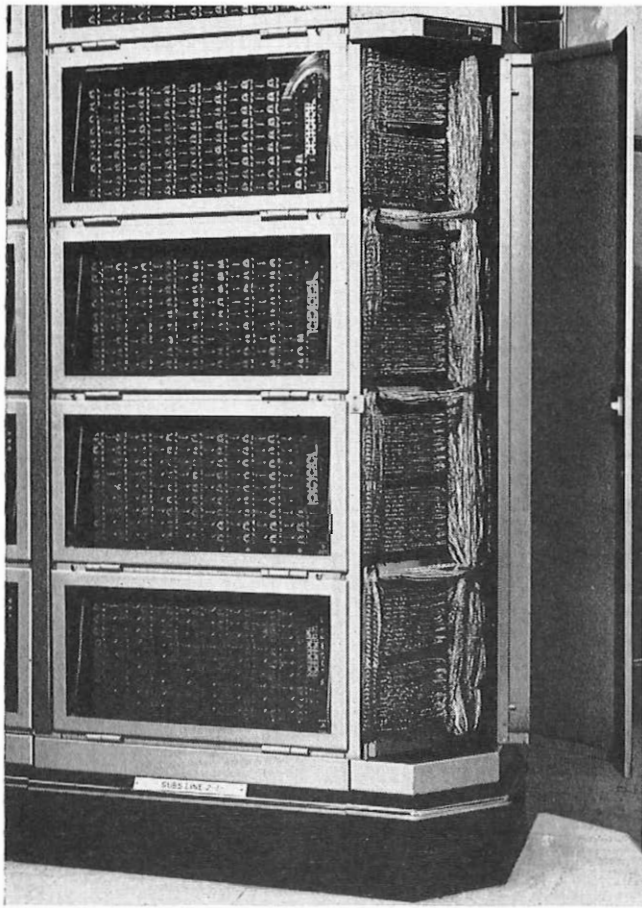
FIG. 11—SUBSCRIBERS' LINE-CIRCUIT RACK AND LINE I.D.F.
