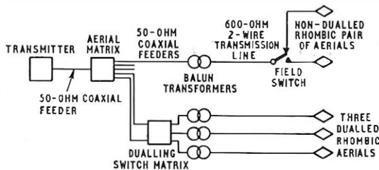
FIG. 1—AERIAL SWITCHING ARRANGEMENTS FOR THE 30 kW SYSTEM
