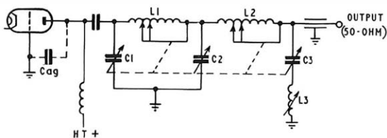
FIG. 5—POWER-AMPLIFIER ANODE AND OUTPUT CIRCUIT
