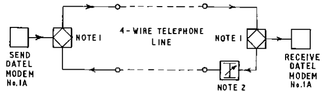
FIG. 5—TEST ARRANGEMENT FOR ASSESSING EFFECT OF SIGNAL ECHO
