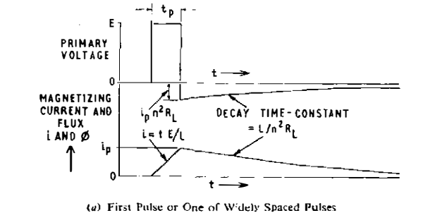
(a) First Pulse or One of Widely Spaced Pulses
