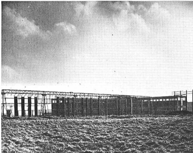
FIG. 3—THE GANTRY FOR 30 kW BALUNS
