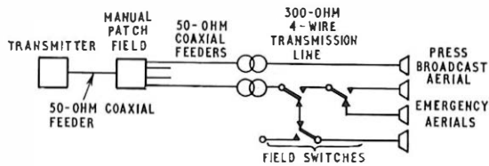
FIG. 6—AERIAL SWITCHING ARRANGEMENTS FOR THE 75 kW SYSTEM
