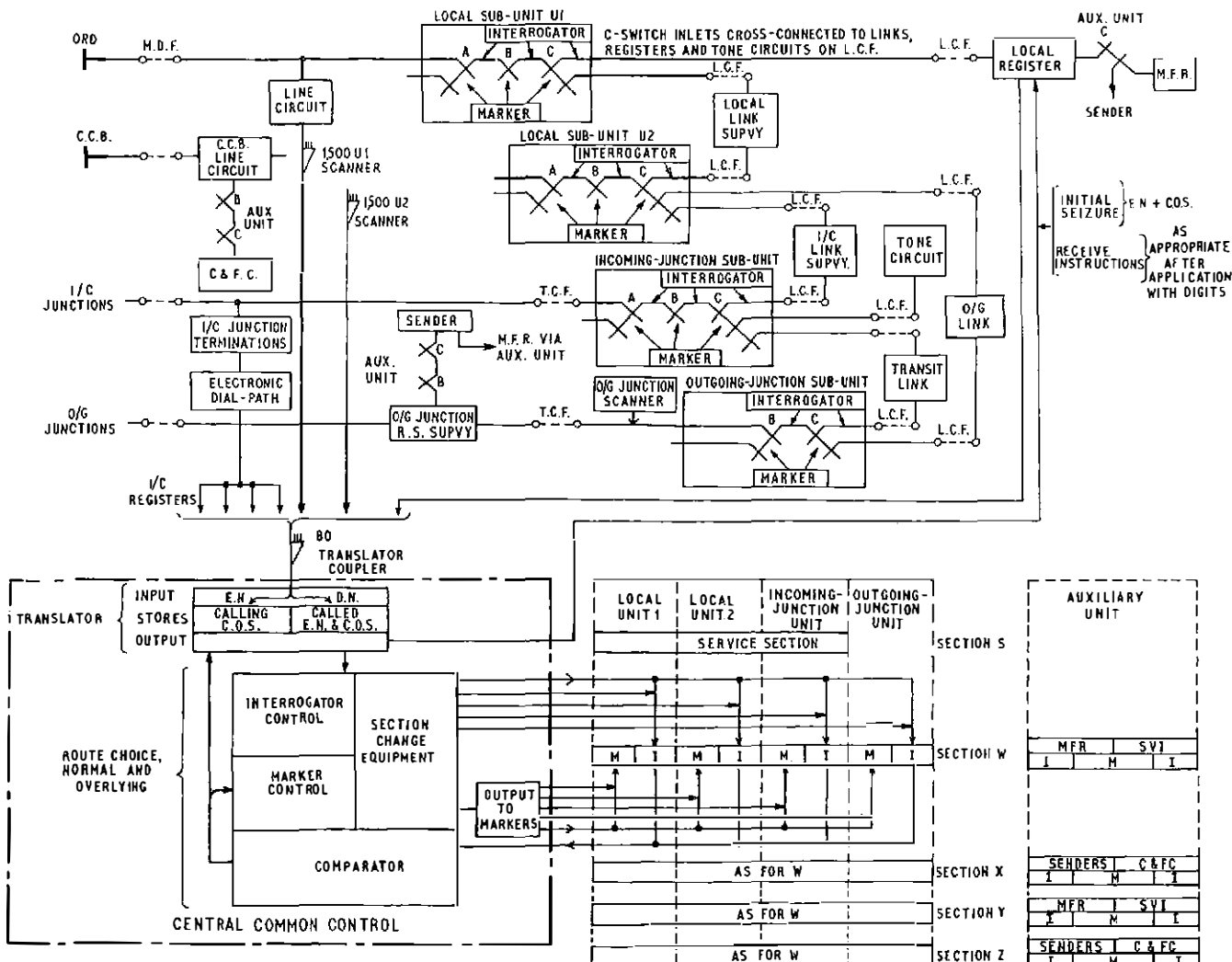
ORD—Ordinary exclusive and shared-service lines. C.C.B.—Coin box. L.C.F.—Link-connecting frame. C. & F.C.—Coin-and-fee-checking circuit. I/C—Incoming. O/G—Outgoing. M.F.R.—Multi-frequency receiver. E.N.—Equipment number. C.O.S.—Class of service. D.N.—Directory number. M—Marker. I—Interrogator. R.S.—Relay-set. SUPVY—Supervisory.
