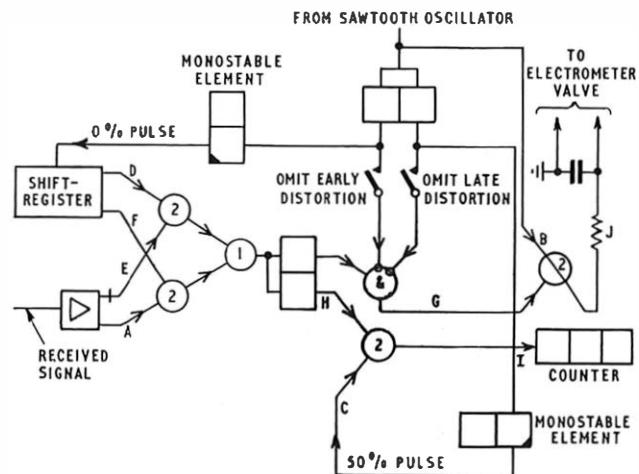
The letters A-J refer to the waveforms shown in Fig. 6. The analogue saw-tooth waveform B is gated by the digital waveform G: this is indicated by the linear-gate symbol. FIG. 7—LOGIC DIAGRAM SHOWING METHOD OF ERROR DETECTION AND DISTORTION MEASUREMENT
