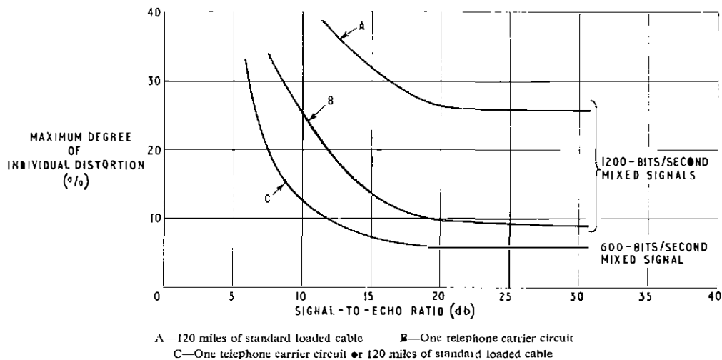
FIG. 6—EFFECT OF LISTENER ECHO ON PERFORMANCE OF DATAL MODEM No. 1A DEMODULATOR
