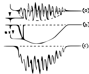
(a) Original Waveform (b) Envelope Component (c) Unilateralized Signal
