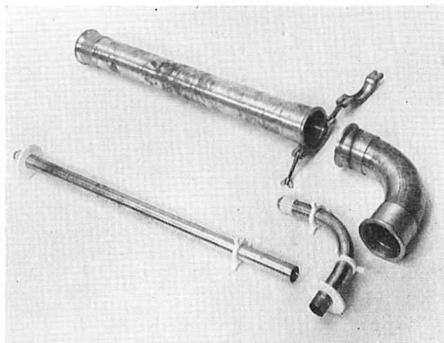
FIG. 7—75 kW COAXIAL-FEEDER COMPONENTS
