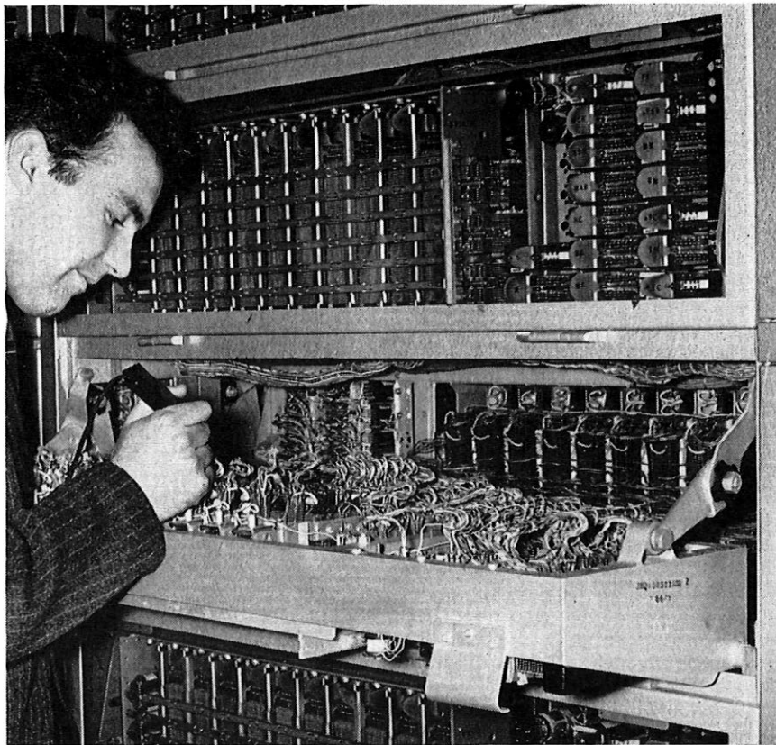
FIG. 12—CHECKING THE WIRING ON A B-DISTRIBUTOR-SWITCH
