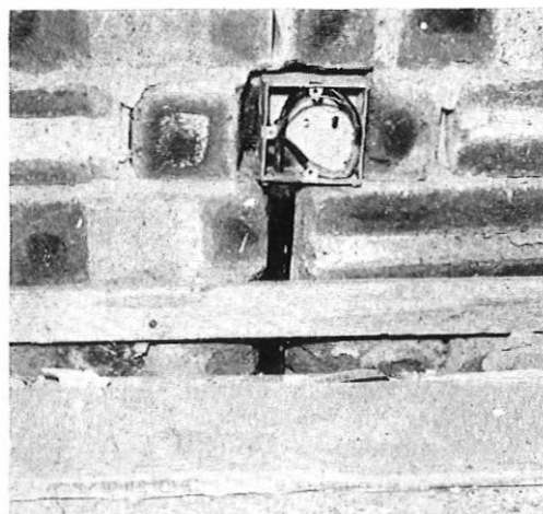
FIG. 1—POST OFFICE CONDUIT BOX IN CHASE IN WALL WITH CABLE AND EARTH WIRE COILED IN BOX
