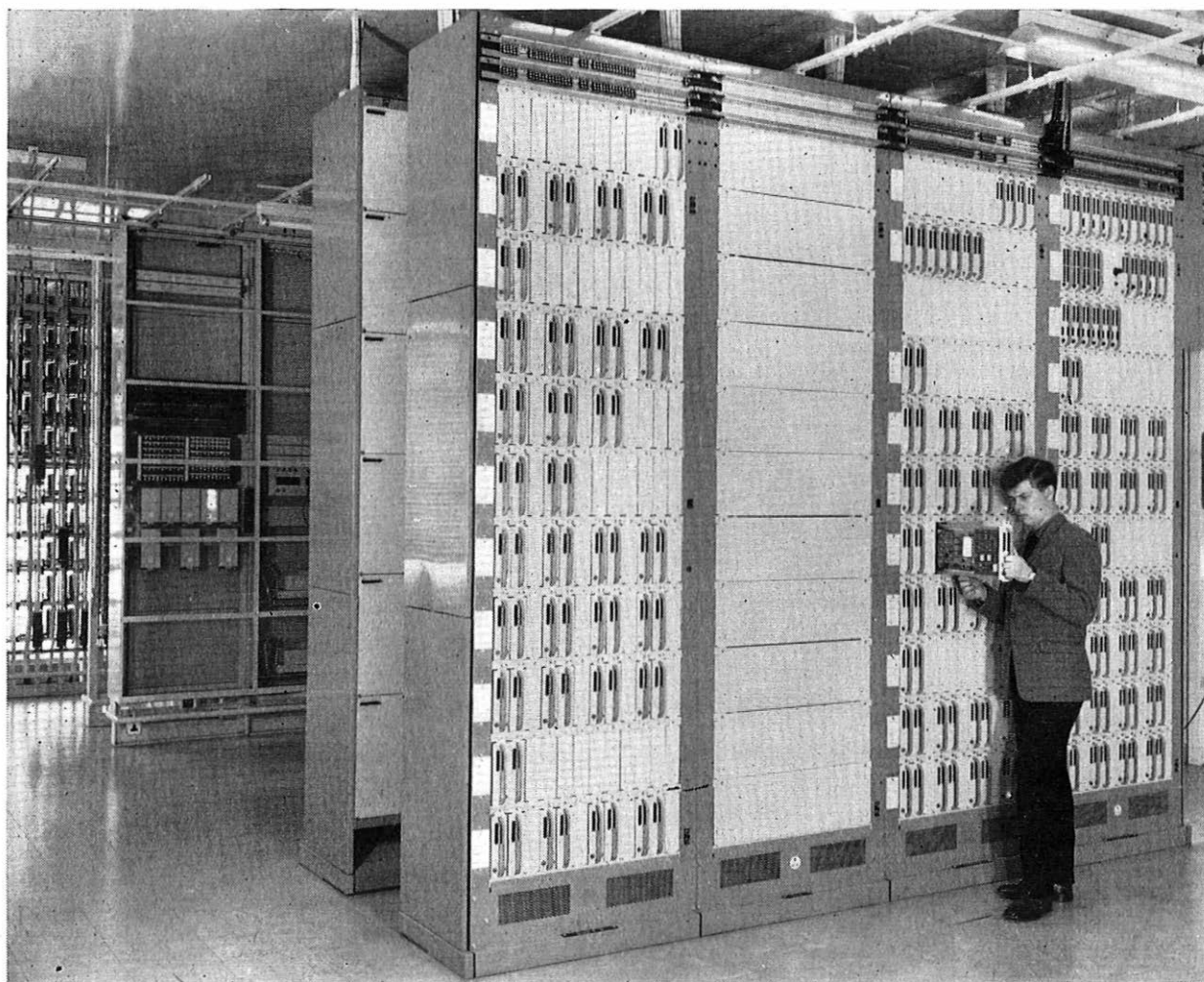
FIG. 2—AMBERGATE ELECTRONIC TELEPHONE EXCHANGE
