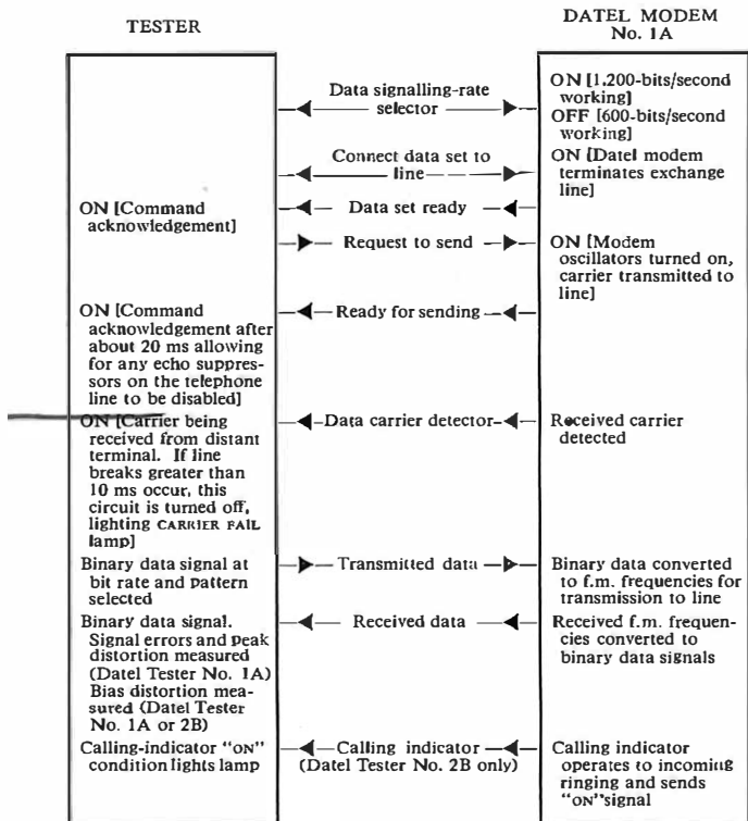
FIG. 1—DIAGRAM SHOWING INTERFACE BETWEEN THE DATTEL TESTER No. 1A OR DATTEL TESTER No. 2B AND DATTEL MODEM No. 1A
