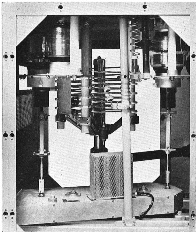
FIG. 4—POWER-AMPLIFIER ANODE-TUNING COMPARTMENT
