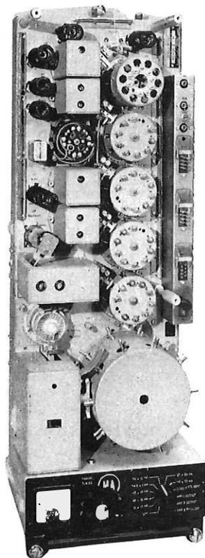
FIG. 2—LOW-POWER AMPLIFIER UNIT
