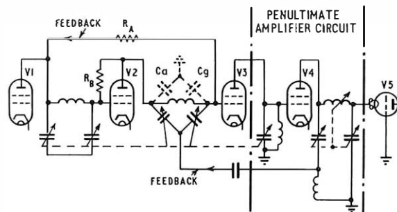
FIG. 3—PENULTIMATE-AMPLIFIER ANODE CIRCUIT AND NEGATIVE FEEDBACK CIRCUITS
