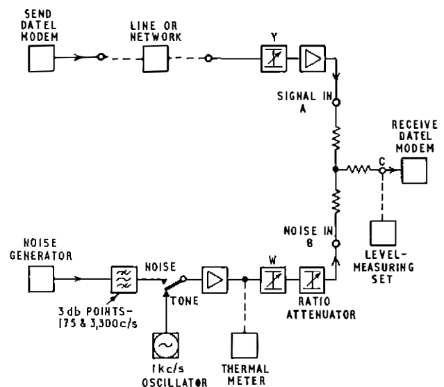
FIG. 1.—LABORATORY-TEST ARRANGEMENT
