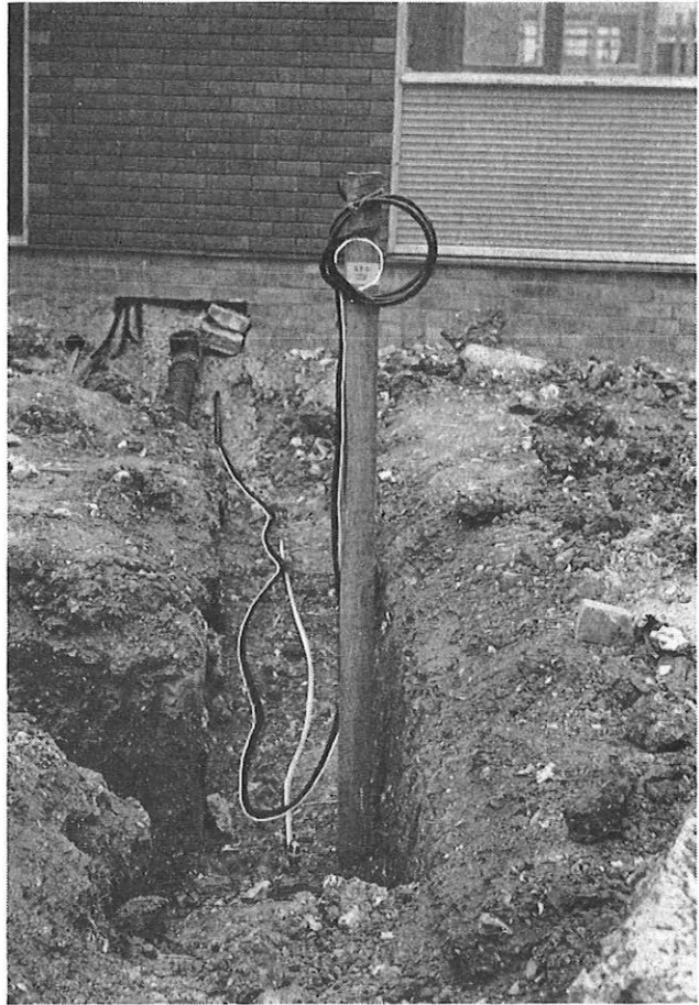
FIG. 3—LEAD-IN CABLE AND EARTH WIRE LAID BY BUILDER IN WATER-PIPE SERVICE TRENCH
