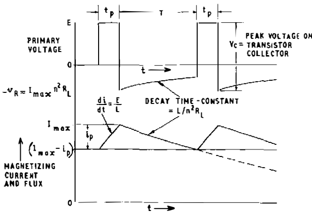
(b) Steady State in Sequence of Pulses
