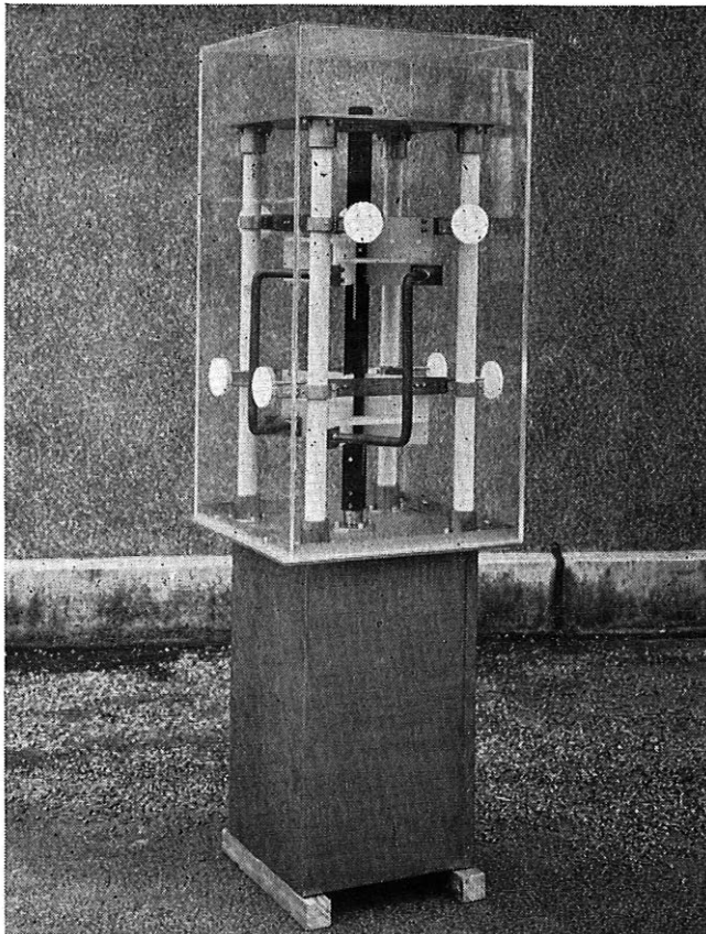
FIG. 9—FIELD SWITCH FOR THE 75 kW PRESS-BROADCAST EMERGENCY AERIALS
