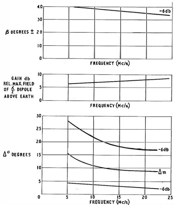
FIG. 10—PERFORMANCE CHARACTERISTICS OF THE LOG-PERIODIC AERIALS
