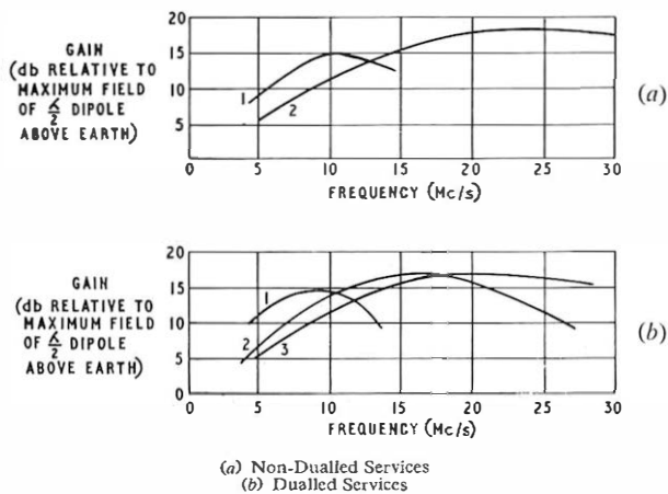
FIG. 5—GAIN CURVES OF THE RHOMBIC AERIALS
