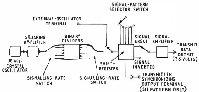
FIG. 3—SIMPLIFIED BLOCK SCHEMATIC DIAGRAM OF DATTEL TESTER No. 1A TRANSMITTER
