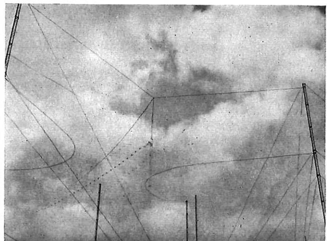
FIG. 11—CONFIGURATION OF THE LOG-PERIODIC AERIAL
