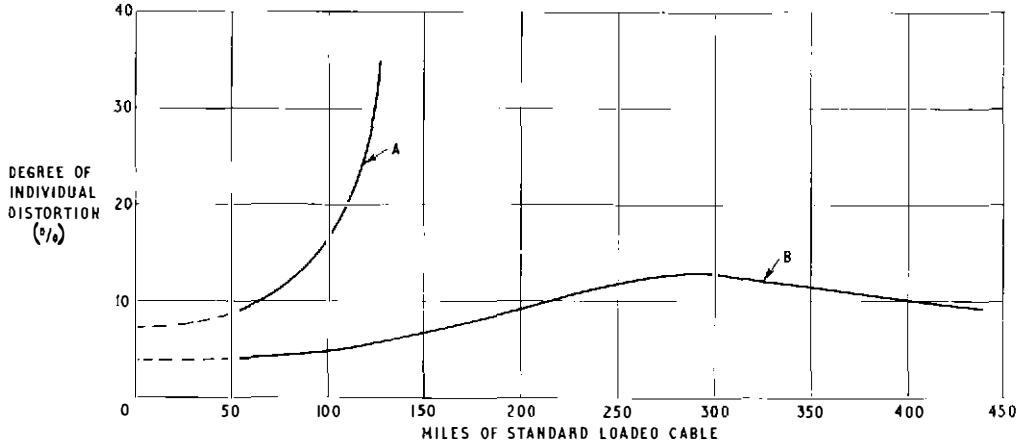
FIG. 3—DEGREE OF INDIVIDUAL DISTORTION RELATIVE TO LENGTH OF CIRCUIT
