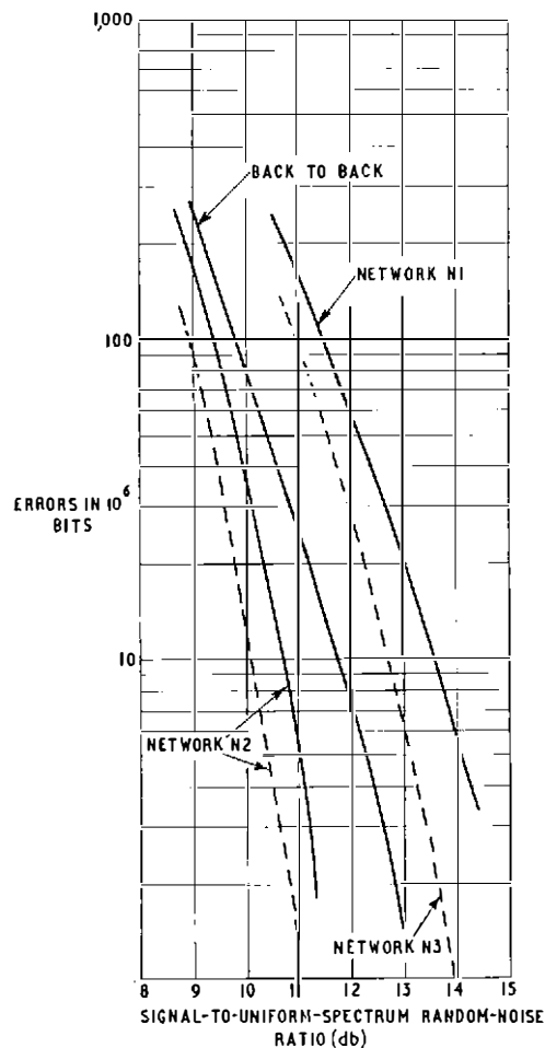
FIG. 2.—RESULTS OF TESTS VIA LINE-SIMULATING NETWORKS
