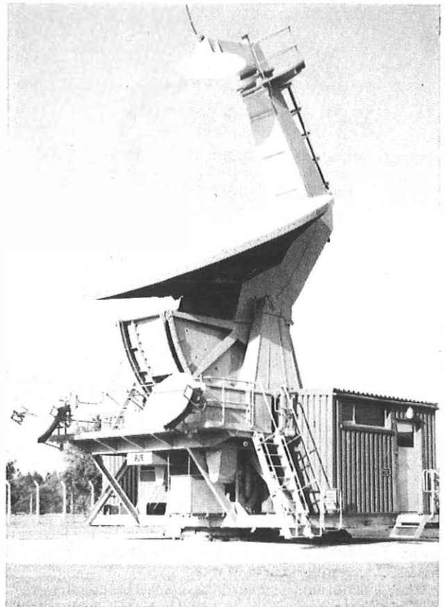
FIG. 10—The Martlesham 6 m diameter steerable aerial
