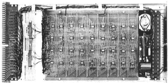
FIG. 10—Empress plug-in unit (1968)
