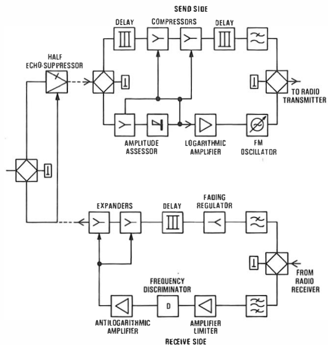
FIG. 8—Block diagram of the Lincompex equipment
