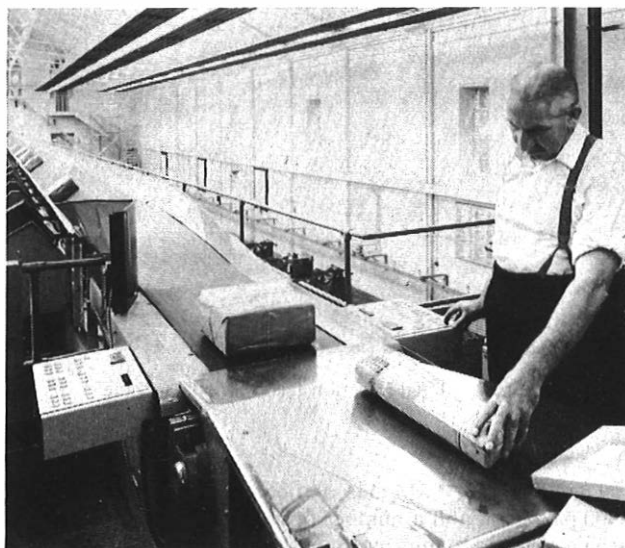
FIG. 1—Tilted-belt parcel sorting machine
