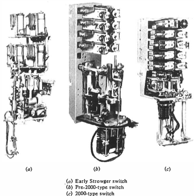
FIG. 1—Strowger 2-motion switches
