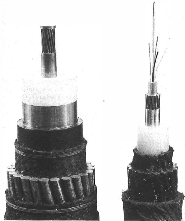
(a) SG -type coaxial cable (43 mm diameter) (b) Loch Fyne optical-fibre cable Note: The SG -type coaxial cable system has a capacity of 4000 circuits. Early optical-fibre cable systems have a capacity of 1920 circuits (140 Mbit/s) per fibre pair. The design shown allows a maximum of 5 pairs
