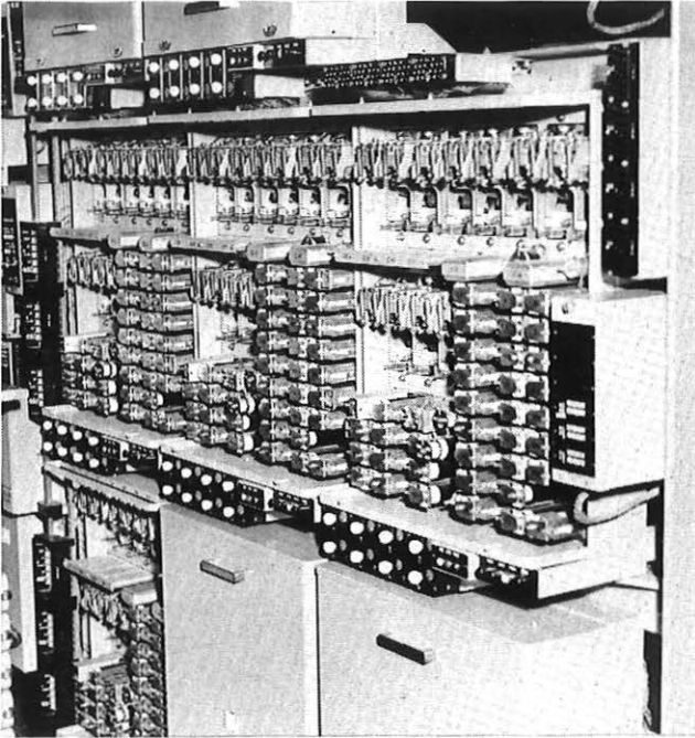
FIG. 1—Electromechanical registers (Evesham 1960)
