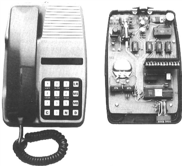
Experimental microprocessor telephone
