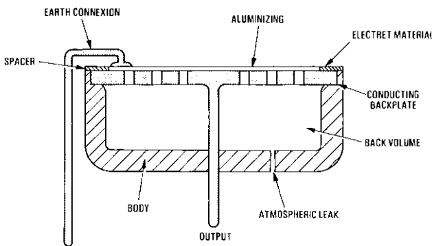
FIG. 4—Simplified cross-section of the electret microphone
