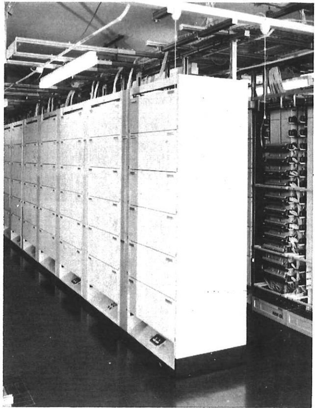
FIG. 9—Baynard House System X equipment (1980)
