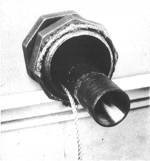
FIG. 11—Millimetric waveguide in its steel duct
