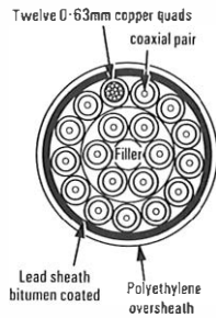
FIG. 7—Cable Coaxial, 18 pr/2·6/9·5 mm + 24 pr/0·63 mm
