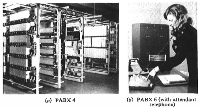
FIG. 11—Strowger-type PABXs
