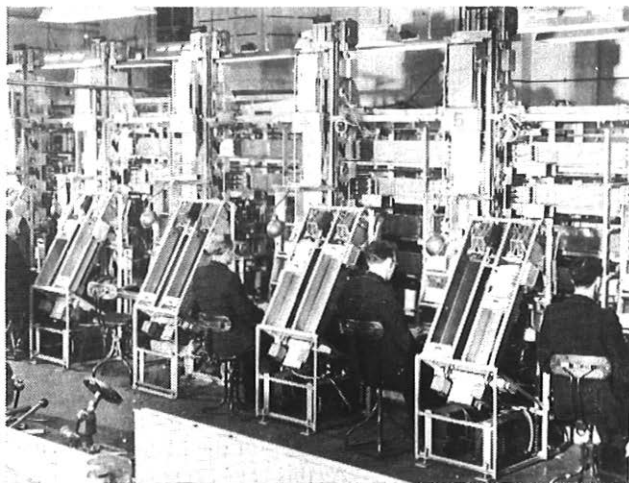
FIG. 1—The 6-position letter-sorting machine
