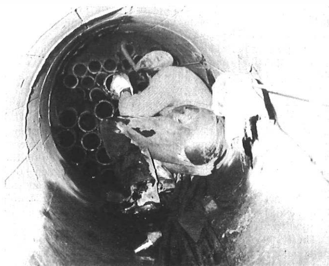
FIG. 14—Ducts being inserted into a mini-tunnel
