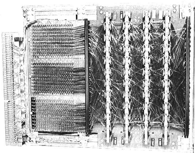
FIG. 9—TXE4 main control unit program store (1975)
