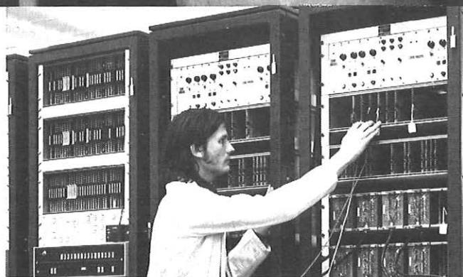
A Postcode translator undergoing final tests before delivery to the Post Office.
