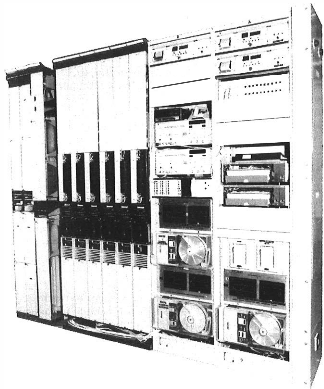
FIG. 1—11 GHz, 140 Mbit/s QPSK field evaluation equipment
