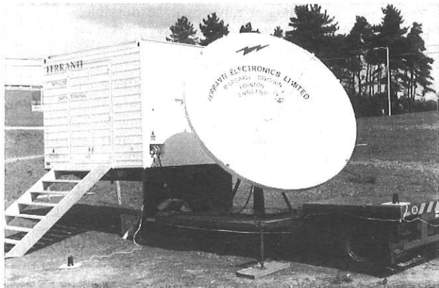
Transportable 3 m small-dish earth station
