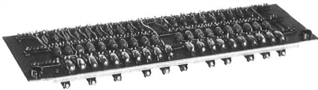
FIG. 4—Typical module of experimental PABX (1955) showing component mounting and interconnexion
