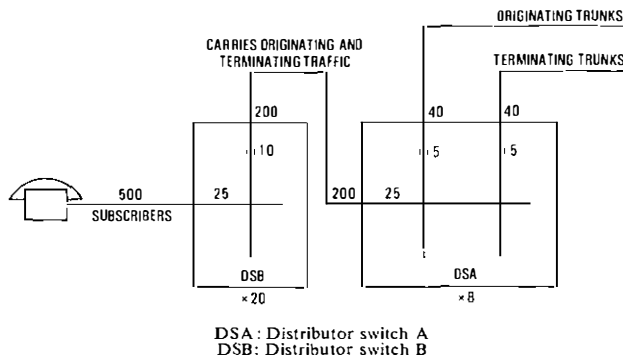
FIG. 3—TXK 1 local distributor stage
