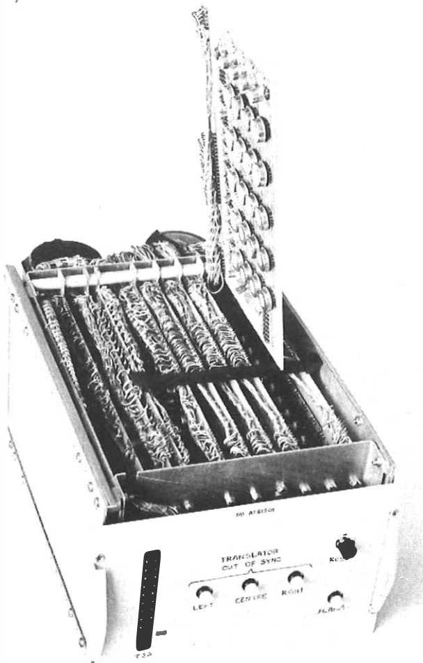
FIG. 7—Type 13 translator with a store card withdrawn
