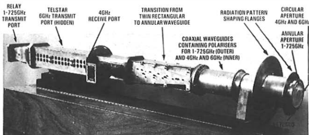
FIG. 9—Composite feed unit for the TELSTAR/RELAY tests
