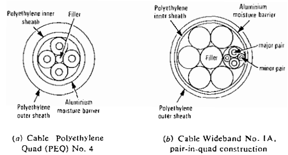
FIG. 5—Special-purpose cables
