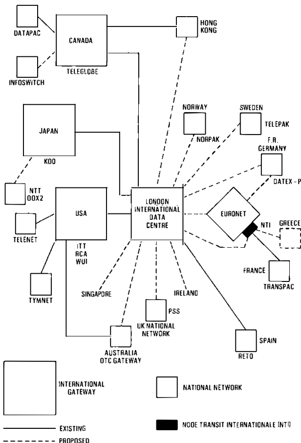
FIG. 2—The planned UK international packet-switched service
