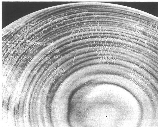
FIG. 25—An X-ray reflection topograph of part of a 50 mm slice of monocrystalline silicon
