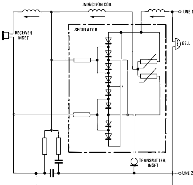
FIG. 3—The transmission circuit of the Telephone No. 706
