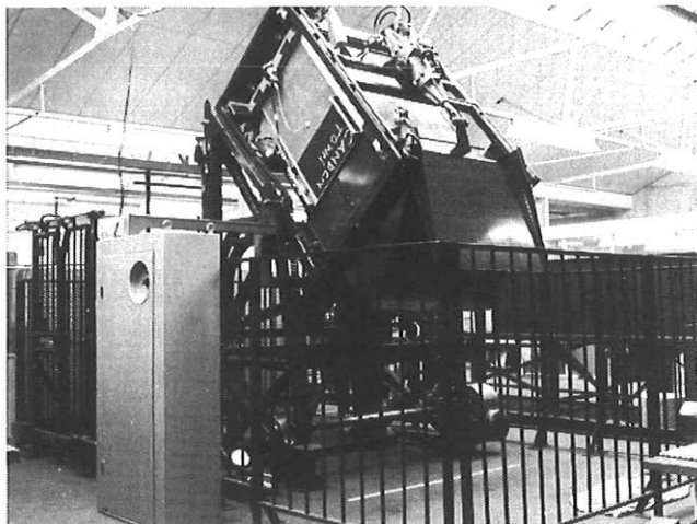
FIG. 10—Lift-and-tip machine
