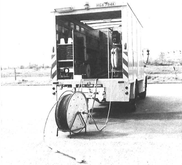
FIG. 17—Rodding and Light-Cabling Vehicle with duct motor in foreground
