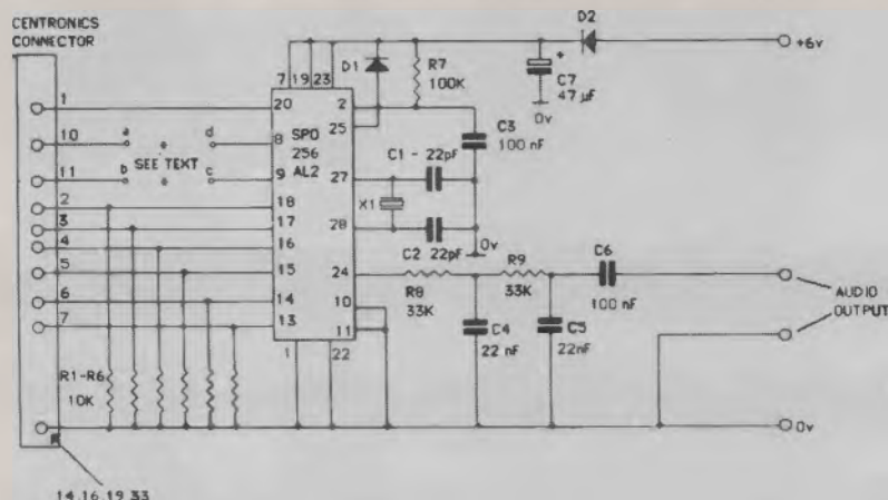
Diagram 2a Speech synthesiser circuit
