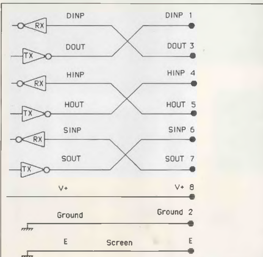
Fig 3b Interconnecting captive cable from an S to D device
