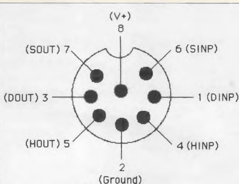
Fig 2 Pin numbering of 8-way DIN socket (front view)
