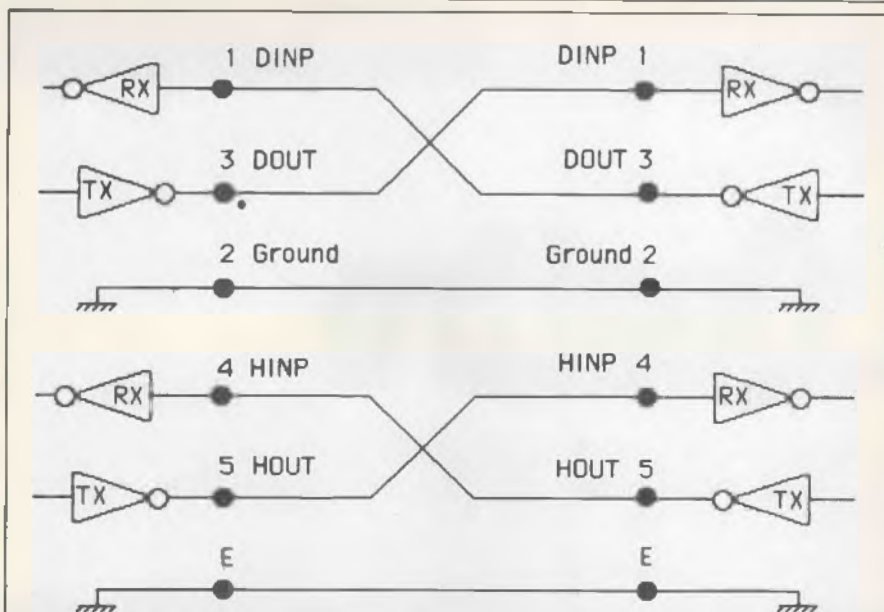
Fig 3a Interconnecting cable for a D to D device
