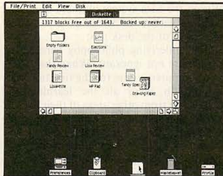
Figure 2. Moving the pointer over the diskette icon with the mouse and clicking it opens up the diskette icon into a window revealing what is on the diskette.
