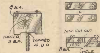
Fig. 4.—(Left) The top clamp. (Right) The bottom clamp.
