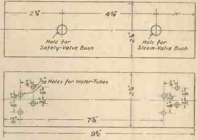
Fig. 5.— Top and underside views of the boiler barrel.
