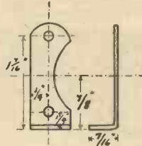
Fig. 7 (right).—Details of the brass brackets, four of which are required.
