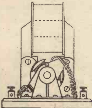
Fig. 1.—An end view of the electric motor.
