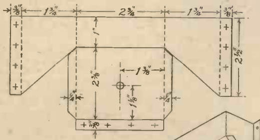
Fig. 8 (above).—How to mark out the plate for forming the chimney support. Fig. 9 (right).—The chimney support bent to shape.
