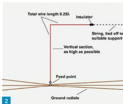
Fig. 1: The 22.5m (74ft) base-loaded vertical for 160m at PJ4DX. Fig. 2: Basic design of quarter-wave inverted-L antenna. Fig. 3: Excerpt from 160m Logbook of The World record.
