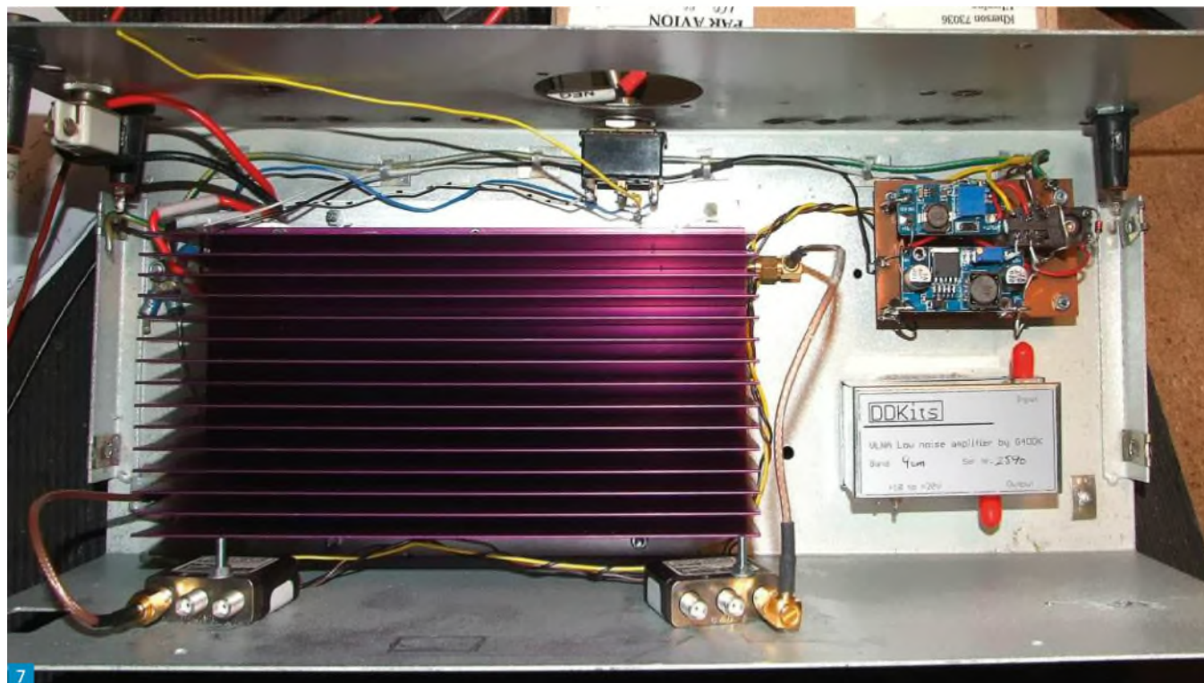
Fig. 7: The 9cm PA and LNA being boxed.
