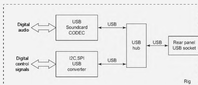
Fig. 5: Typical audio/CAT internal block diagram of a digital rig.
