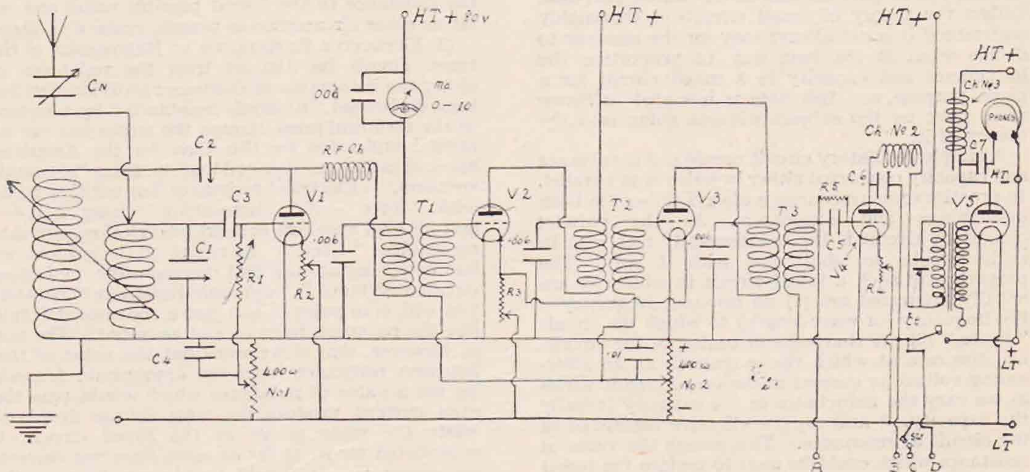
FIG. 2. DIAGRAM OF S/W SUPER-HETERODYNE. FIVE VALVES WITH LONG-WAVE OSCILLATOR. A 30-ohm rheostat should be connected in series with the negative contact of potentiometer No. 2 and L.T.—bus bar—this gives a good vernier control over I.F. oscillation point.
