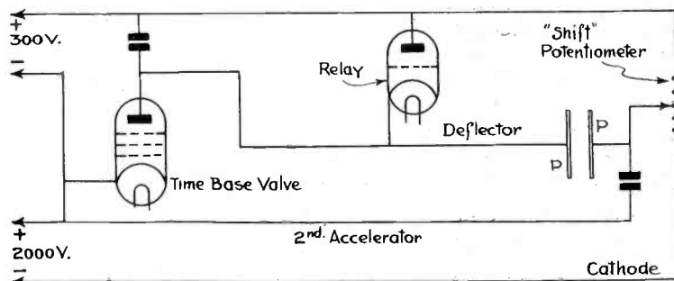
Fig. 3.—Showing how the deflector plates P differ appreciably in potential from the second accelerator. This causes de-focusing of the beam on parts of the screen.
