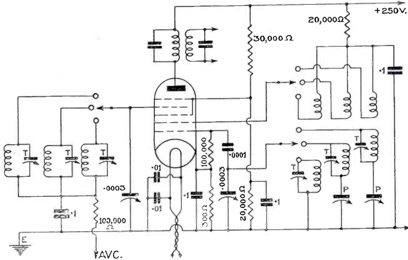
Fig. 1.—This is the heart of an efficient short-wave super-het. It can be added to almost any short-wave super but preferably one with 450 kc. I.F. transformers.
