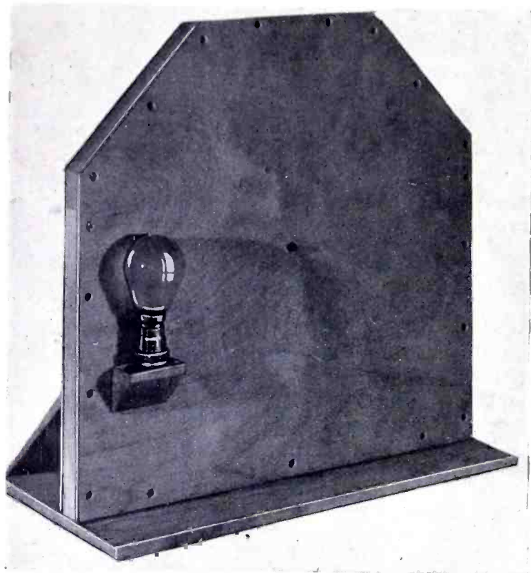
Photograph of the back of the receiver.
