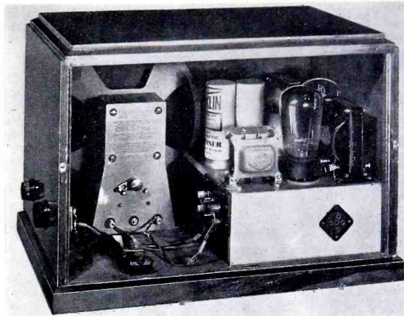
Most of the wiring is point to point. This is most essential on the higher frequencies. Keep the connecting wires short.
