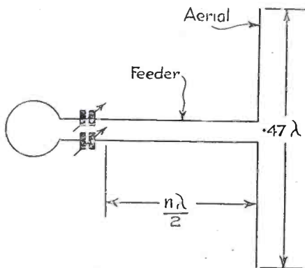
Fig. 5 (right).—Theoretical circuit of transmitter.
