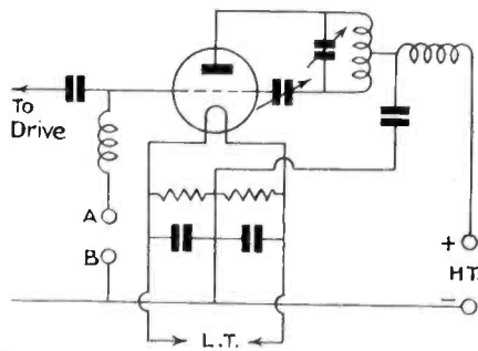
Fig. 4.—With this circuit in use the P.A. will operate down to 10 metres with grid modulation.
