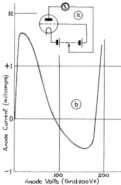
Fig. 1.—(a) Circuit to show secondary emission. (b) Anode current curve for triode with coated anode.
