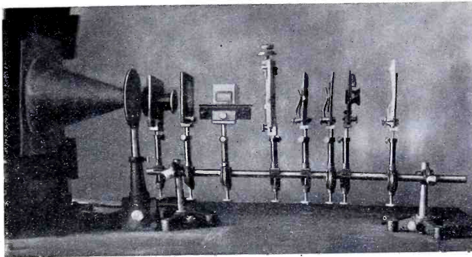
A photograph of the circular polariscope in use.
