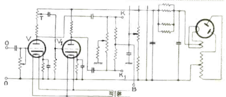
Circuit of push-pull system for cathode-ray tube.
