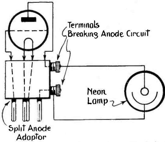
With a commercial receiver a split anode adaptor will come in useful. The lamp can be connected to the two side terminals on the adaptor.
