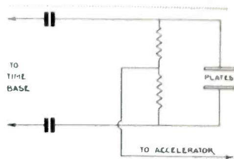
Fig. 5.—Symmetrical circuit for balancing potentials applied to the deflector plates to overcome distortion.
