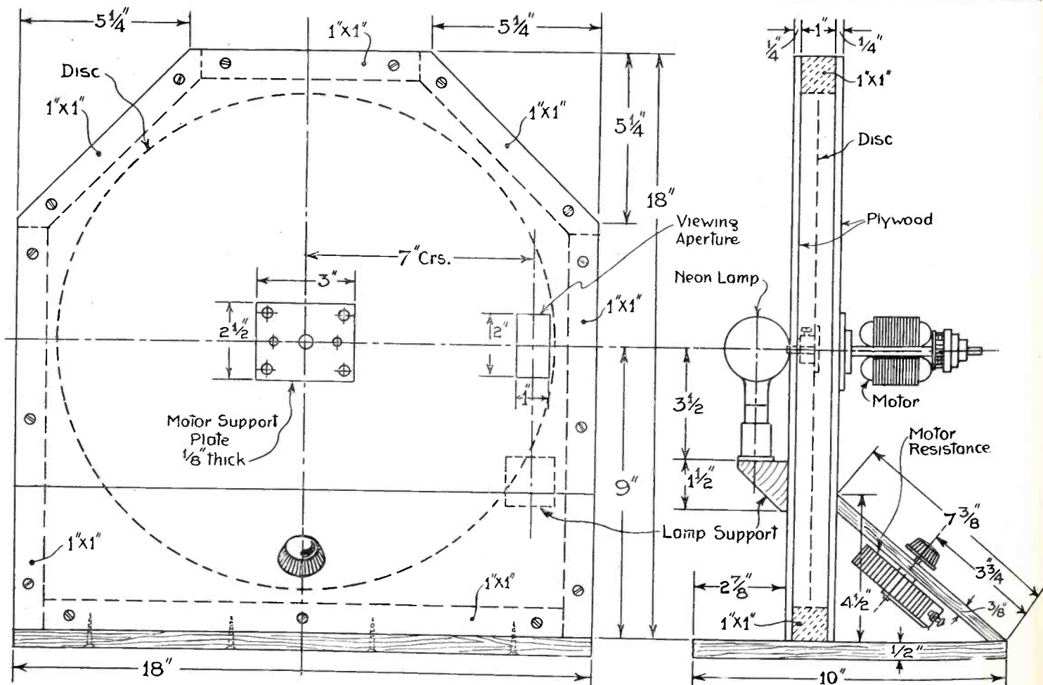
Fully dimensioned drawings of front and end elevations of the receiver. All the necessary constructional details are quite clear.
