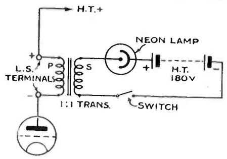
If you have two receivers and can spare one for television, this circuit can be recommended. Simply take off the loud-speaker and connect to neon lamp as indicated.
