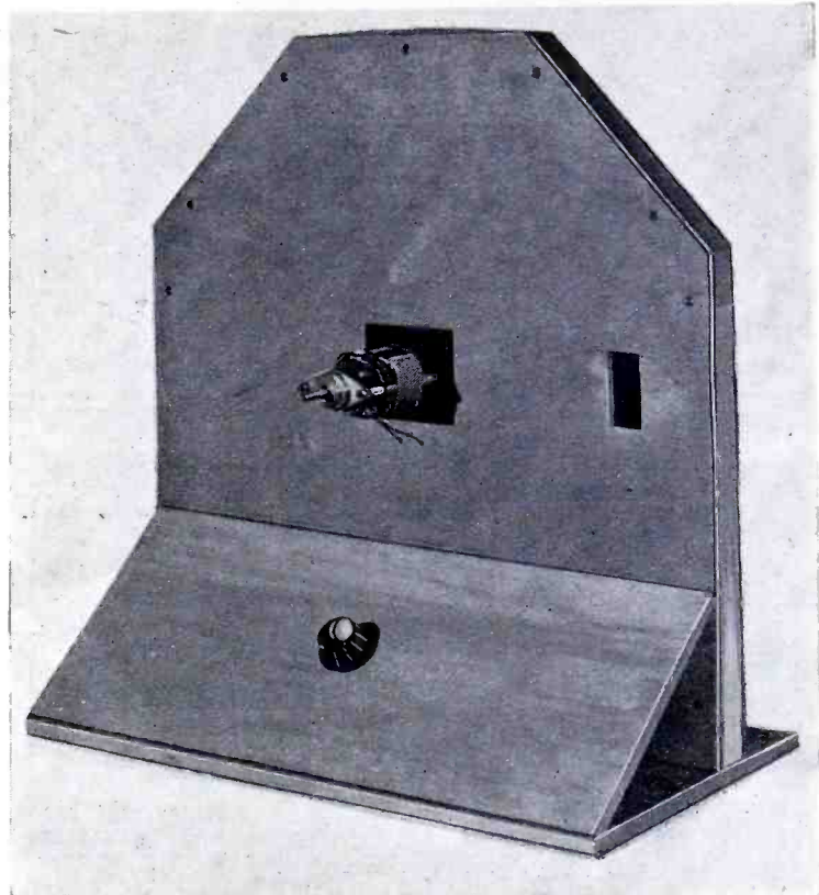
This photograph shows the complete receiver
