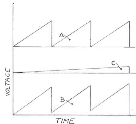
Fig. 2.—Wave-forms for interleaved scanning. Patent No. 423,101.
