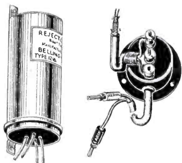
On the left is the first impedance matching transformer connected close to the aerial at the top of the mast. The second transformer is fitted to the receiver chassis.
