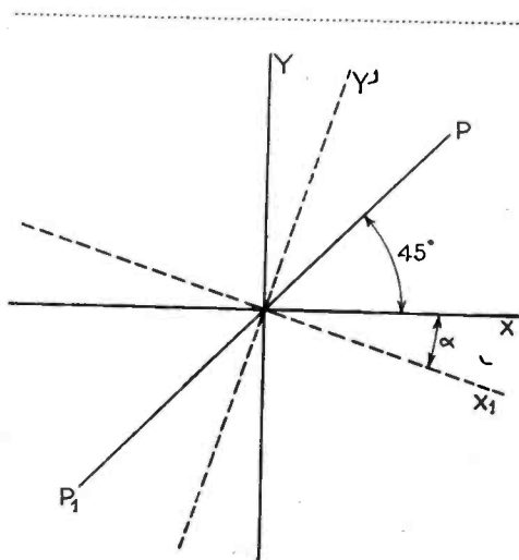
Fig. 2.—The circular polariser and analyser.— PP_1 is the nicol with quarter-wave plate OX ; OX_1 is the analysing quarter-wave plate.
