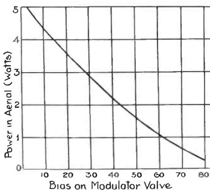
Fig. 6 (left).—Modulation characteristic.
