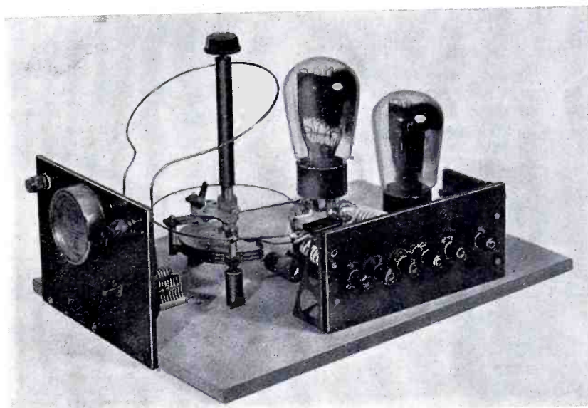
The 7-metre test transmitter.
