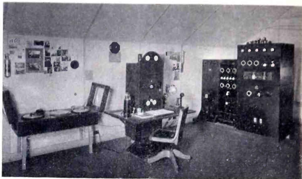
From left to right will be seen recording gear, electric grammo-motor and pick-up, radio receiver, mixing panel, cathode-tube monitor and ribbon microphone, and finally the all-wave band transmitter and class B modulator.
