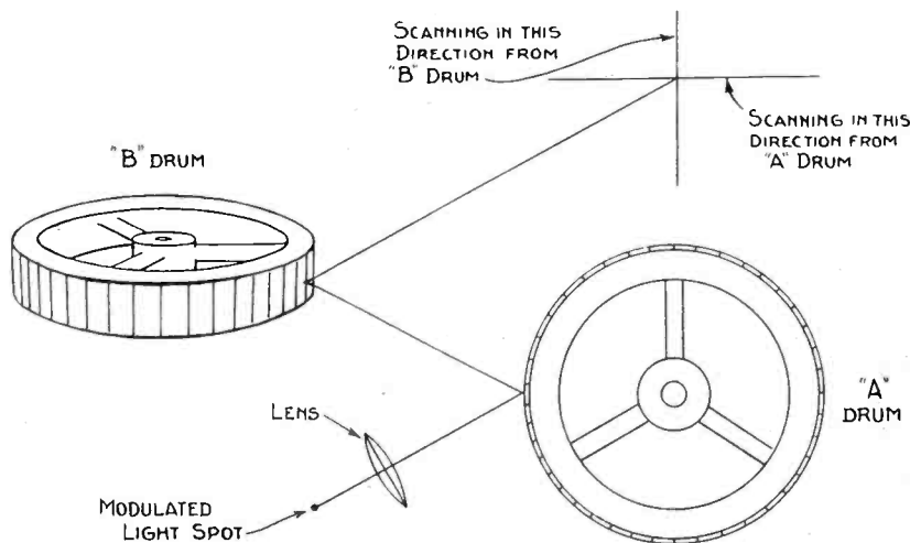
A suggested scheme for high-definition mechanical scanning employing two mirror-drums.
