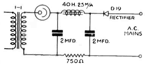
It is an expensive hobby running a neon lamp from dry batteries, so if you have mains laid on use a metal rectifier of the half-type wave. Don't forget the small resistance in series with one side of the supply.
