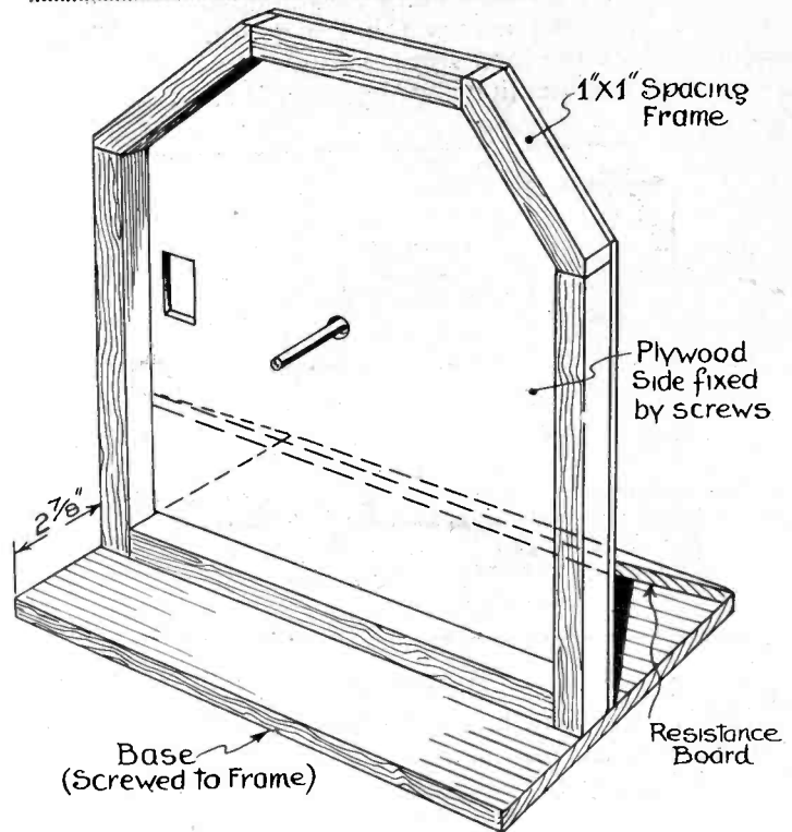
This drawing shows the partly assembled case.
