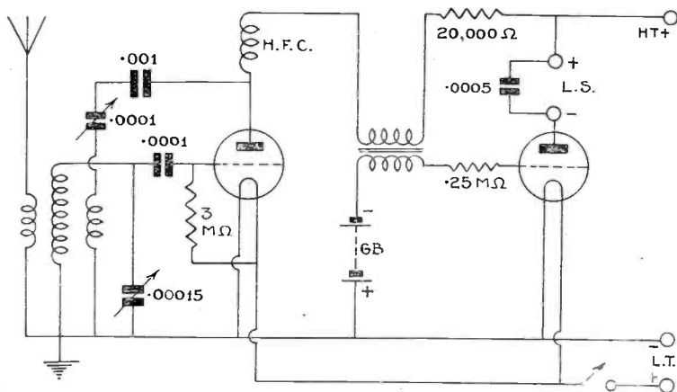
Here is the circuit for the Beginners' Two . There is only one high-tension voltage tapping; it is impossible to short-circuit high-tension to the reaction condenser owing to the use of a series blocking condenser.
