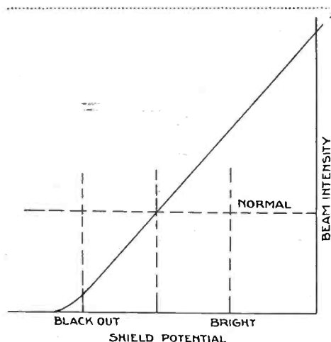
Fig. 1.—Ideal curve of beam intensity—shield potential giving full modulation with no distortion.
