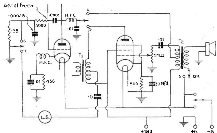
Who will be the first amateur to experiment with micro-waves? This circuit will be a good one with which to start.
