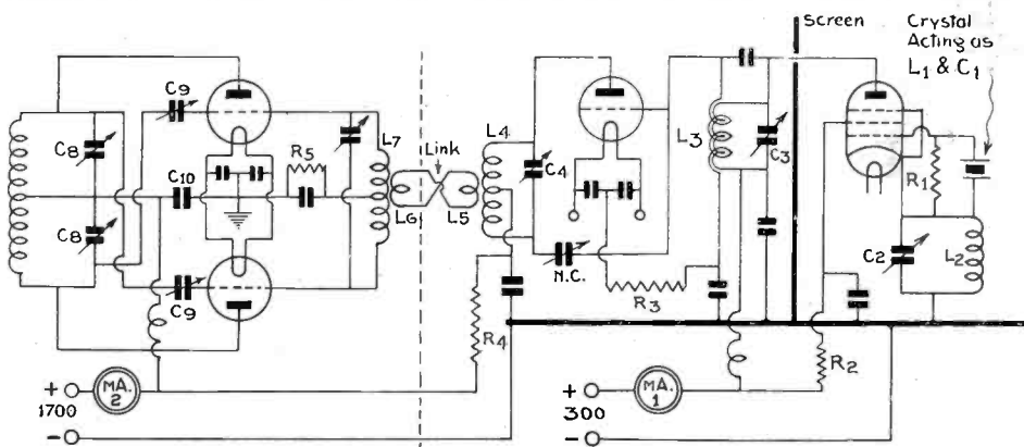
It is a sound idea to couple the CO to the sub-amplifier by means of a transformer. This does overcome the possibility of a faulty high-frequency choke.
