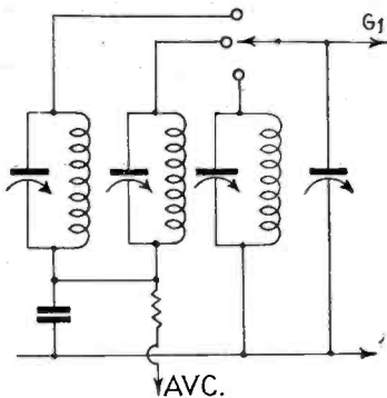
Fig. 2.—It is suggested that on the 25-megacycle band automatic-volume control be omitted. Notice that the third coil is then connected to earth.
