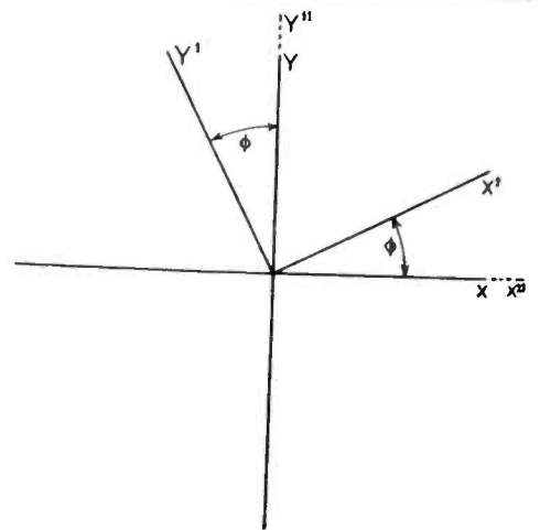
Fig. 3.— OX =fast direction of first quarter-wave plate; OX_1 =fast direction of birefringent section; OX_2 =fast direction of analysing quarter-wave plate.
