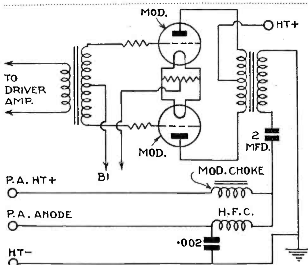
Try push-pull to increase the modulation percentage. There is not any need to alter the P.A. circuit with this arrangement.
