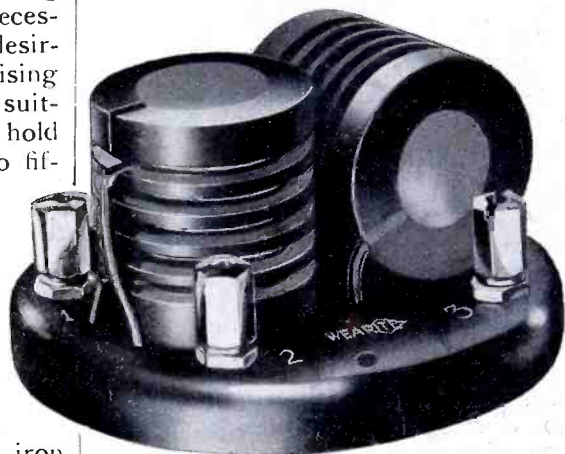
The Wearite wave-trap coil.
