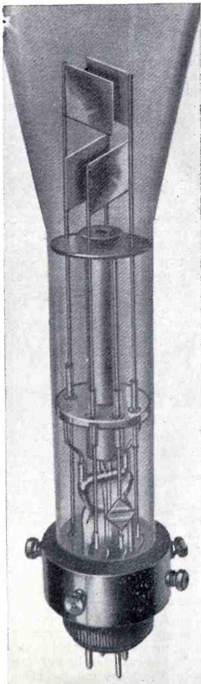
Fig. 1.—Photograph of the electrode assembly of the cathode-ray tube.
