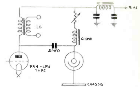
This is a circuit that can be used with the mains receiver. If the applied voltage is too high, the definition will suffer. This can be overcome by the use of the variable resistance.
