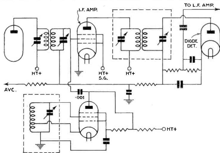
Fig. 1.—By feeding the output from a beat note oscillator into the grid of an I.F. amplifier, C.W. reception is considerably simplified. No super-het receiver without an oscillator of this kind is suitable for C.W. reception.
