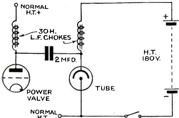
If a choke filter circuit is favoured it can be linked up to the lamp in this way.
