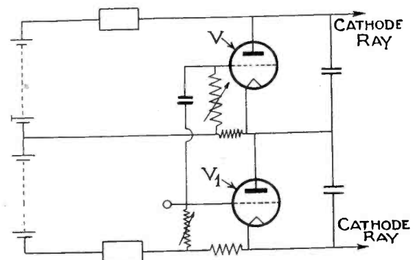
Fig. 1.—Circuit for producing interleaved scanning. Patent No. 423,101.
