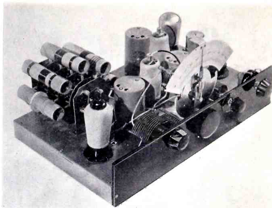
Here is the receiver chassis. The panel is only a temporary one used to secure the tuning components during testing.
