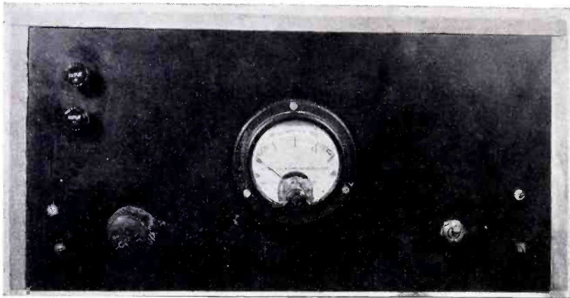
This photograph shows the panel of the valve voltmeter with the sensitivity control at the left.
