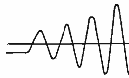
Fig. 15. Unstable closed loop system
