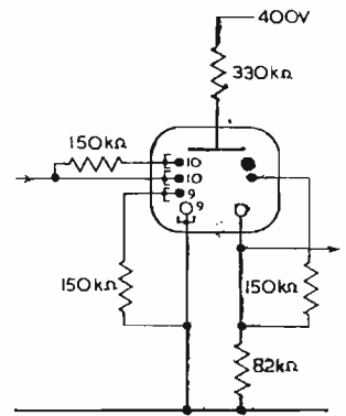
Fig. 9. Circuit showing recommended values
