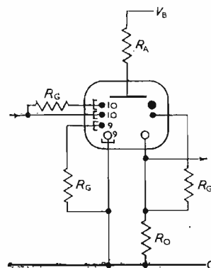
Fig. 8. Circuit referred to in tentative specification
