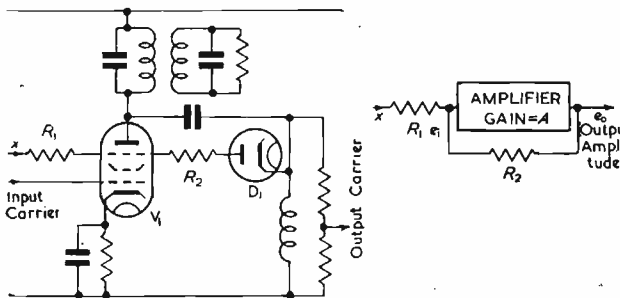
Fig. 2. Circuit for amplitude modulation Fig. 3. Equivalent circuit
