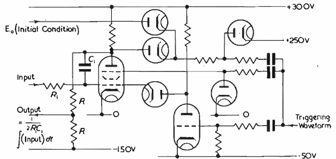
Fig. 9. The integrating circuit
