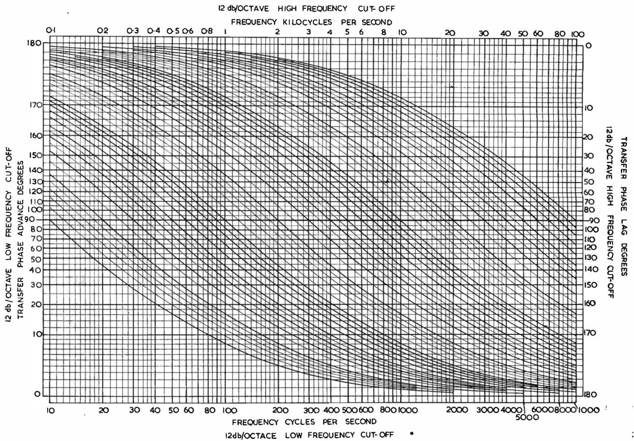
Chart 13. Phase response
