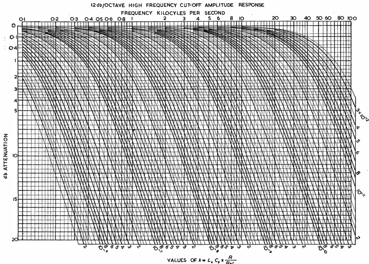
Chart 12. 12db/octave high frequency cut-off
