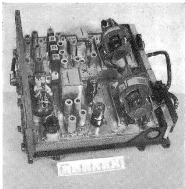
The Transmitter/Receiver Unit of the ship's equipment
