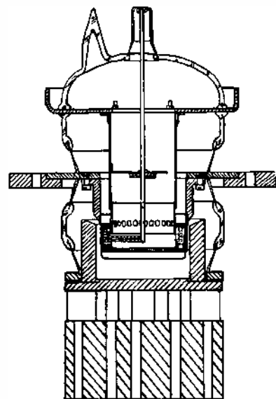
Fig. 6 Cross section of the CV288 disk-seal triode
