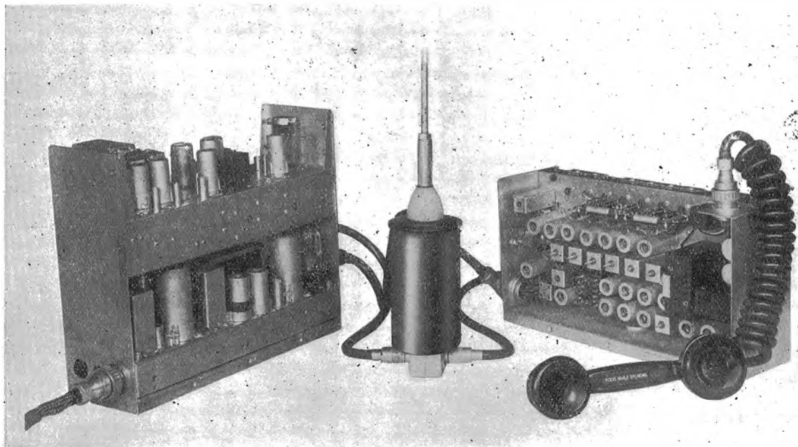
Fig. 5. Equipment for motor-cycle fitting, shown without cases and mountings. On the left is the transmitter and power unit, in the centre is the matching unit fitted in the base of the half-wave aerial, and on the right is the receiver
