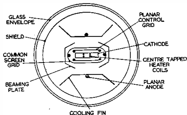
Fig. 3 (right). Crosssection of electrode assembly of the 6QV6-40
