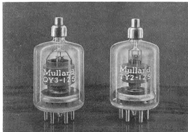
Fig. 4 (left). Two typical power valves in the hard glass V.H.F. range (about \frac{1}{3} rd actual size)
