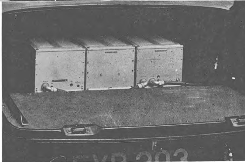
(Bottom right). Installation of three-unit F.M. equipment in boot of patrol car.
