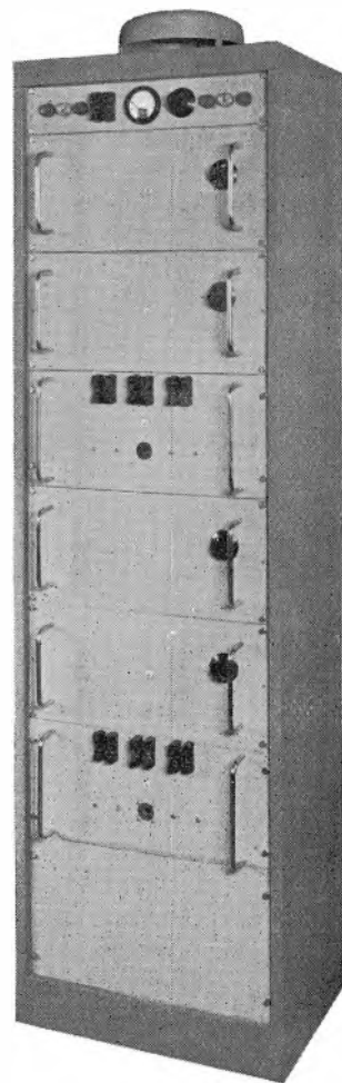
Fig. 4. Two 50 watt transmitters mounted in single cabinet
