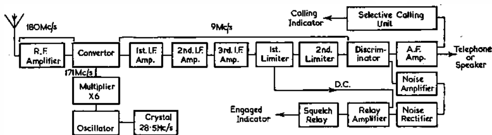
Fig. 1. Block Schematics showing differences between F. M. and A.M. receivers
