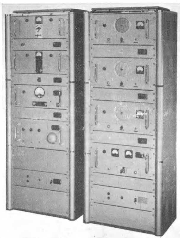
The Control Station Equipment at the Motherwell Station of the Lanarkshire Fire Authority, showing Link Transmitters and Receivers
