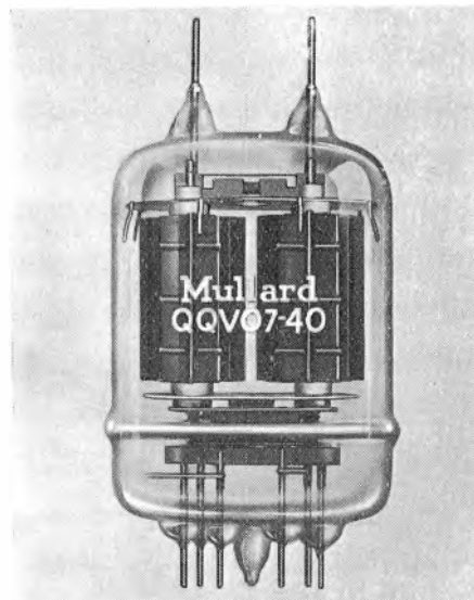
Fig. 1. The QQV07-40 (829B) Double Power Tetrode ( \frac{1}{2} th actual size)
