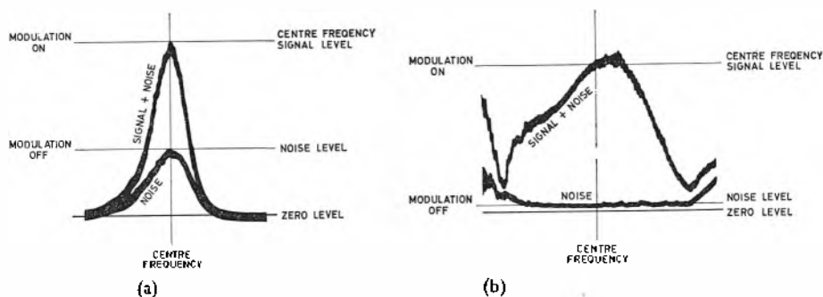
Fig. 9. Oscillograms of mod-on/mod-off displays for noise-limited sensitivity measurement on a.m. and f.m. receivers.
