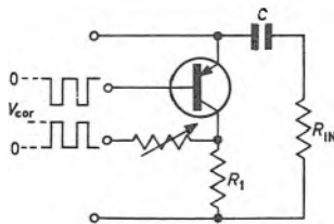
Fig. 5. Method of introducing a correcting waveform to eliminate the initial offset
