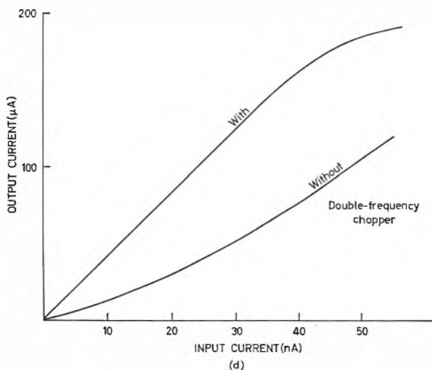
Fig. 9. Performance of a practical chopper amplifier
