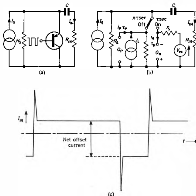
Fig. 4 (a). Current amplifier chopper with blocking capacitor at output
