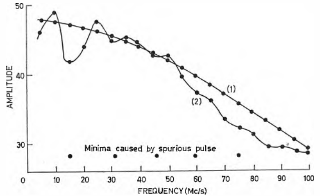
Fig. 8. Fourier spectrum of fast pulse and effect of spurious pulse Curve 1 Time-base speed = 1nsec Curve 2 Time-base speed = 10nsec Length of spurious pulse = 65μsec Zeros in spectral contour = n/65\text{nsec} = n/15\text{Mc/s} n = 1, 2, 3
