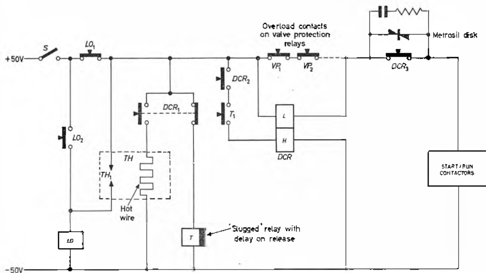
Fig. 9 (above). Basic circuit of d.c.r. with 'line' and 'holding' coils
