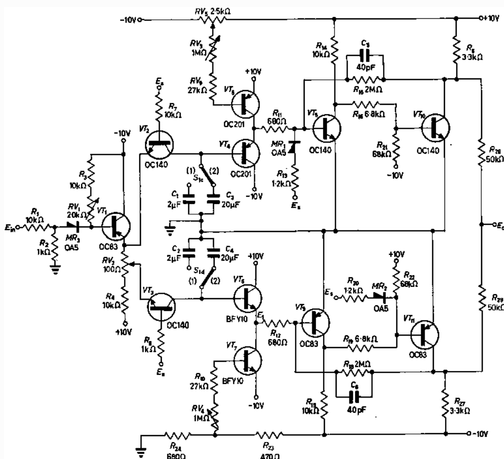
Fig. 4. Pulse-width modulator circuit
