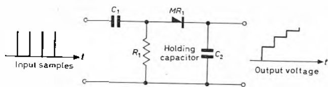
Fig. 6. Basic holding circuit
