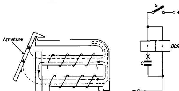
Fig. 1 (left). Shunt field relay Fig. 2 (right). Capacitor in series with one coil
