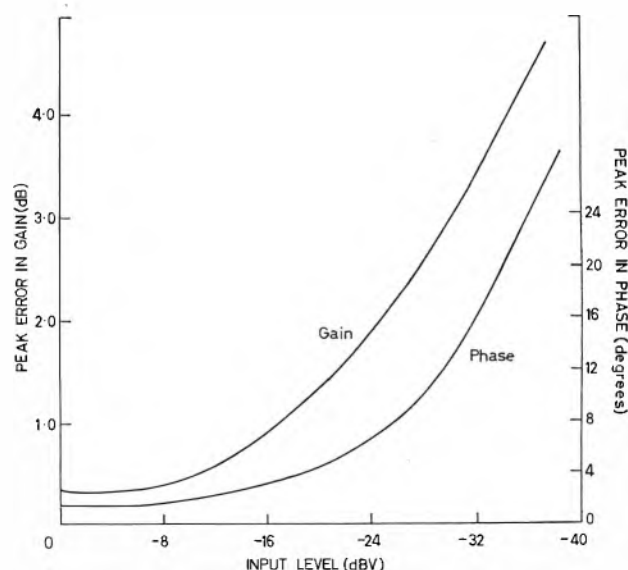
Fig. 19. Effect of quantization noise on accuracy
