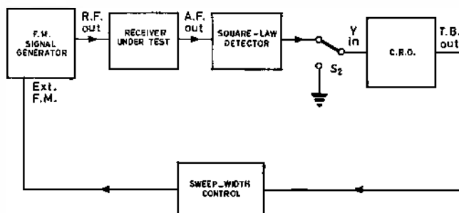
Fig. 5. Arrangement for sensitivity measurement
