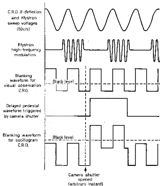
Fig. 3. Switching, sweeping, and blanking waveforms
