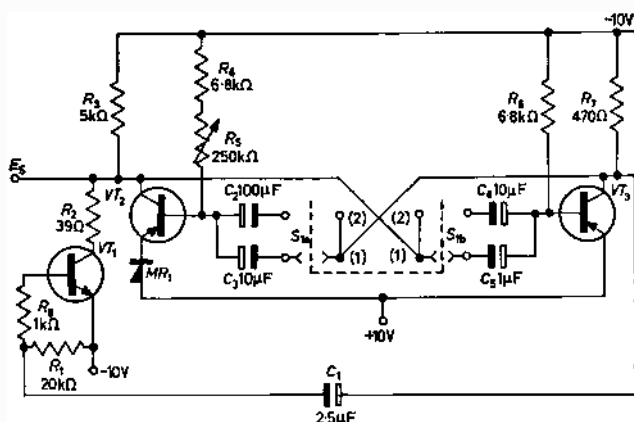
Fig. 3. Sampling interval multivibrator
