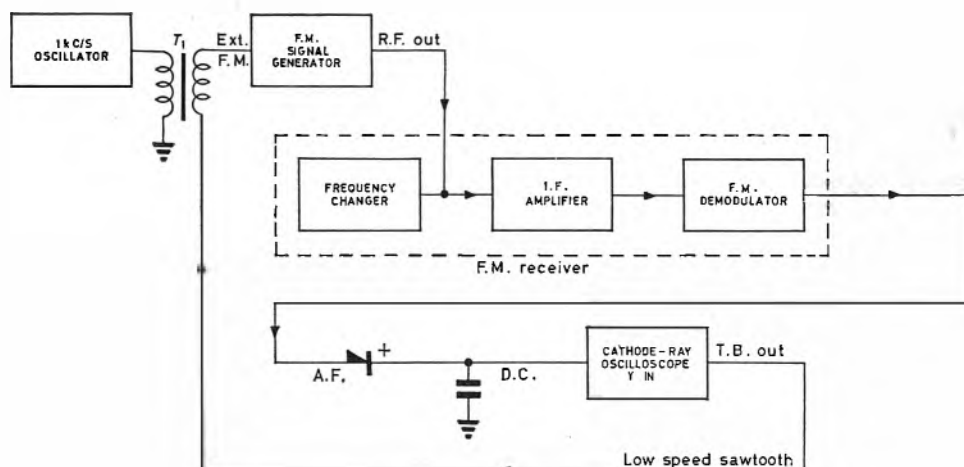
Fig. 8. Connexions for displaying derivative curve. For sensitivity measurement, the r.f. output of the signal generator is applied to the aerial input of the receiver
