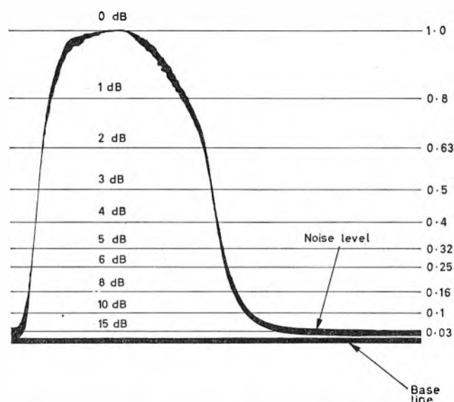
Fig. 6. The sensitivity-measurement display for single-sideband receiver. The baseline with the input short-circuited is also shown on the photograph
