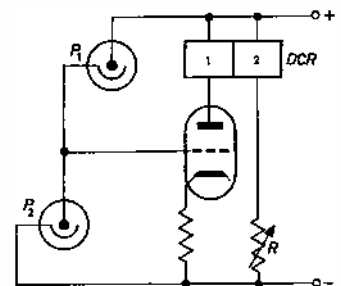
Fig. 4 (above). (a) Relay to operate on incident light (b) Relay to operate on extinction of light
