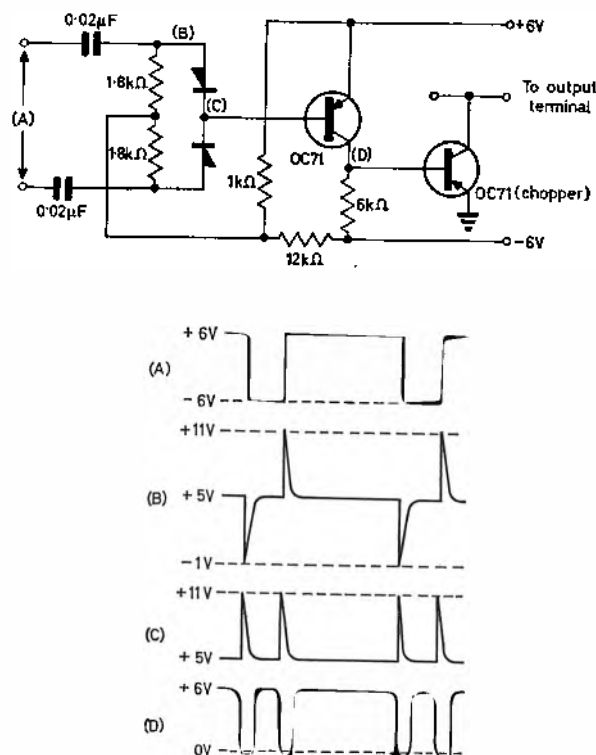
Fig. 8. Circuit and waveforms of a double-frequency chopper designed to eliminate the input positive transient
