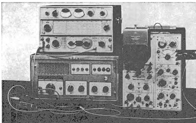
Fig. 3. Test arrangement comprising a Marconi TF2002 signal generator and TF2200A oscilloscope for dynamic display of response characteristics
