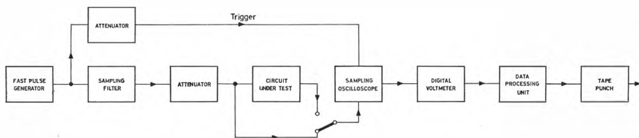
Fig. 4. Experimental model
