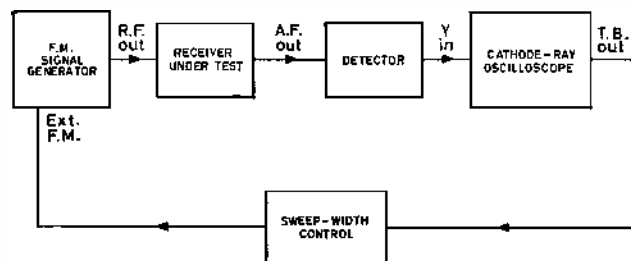
Fig. 1. Basic arrangement for using a frequency modulated signal generator for dynamic display of frequency response characteristic
