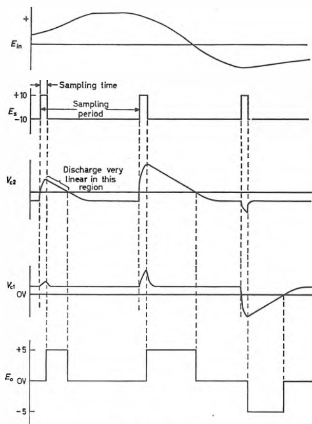
Fig. 5. Typical waveforms
