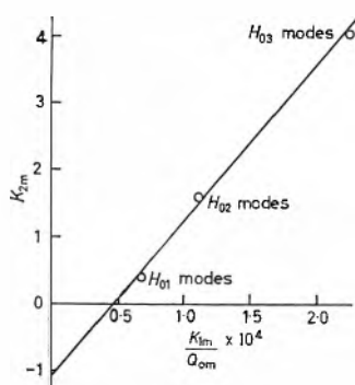
Fig. 4. K_{2m} versus K_{1m}/Q_{0m} for the H_{0mn} series of modes
