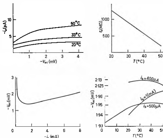
Fig. 3. Variations of switching errors in an OC203
