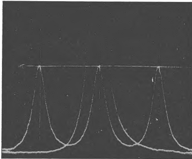
Fig. 2. Typical oscillogram: response shown is for H_{11,226} resonance in 1-metre cavity of 2in diameter plain copper waveguide Frequency spacing of calibrating peaks: 250kc/s Resonant frequency: 34.935Gc/s Q -factor: 5.4 \times 10^3
