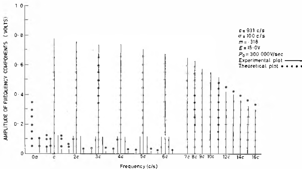
Fig. 4. Experimental and theoretical frequency spectra of trailing edge variable slope modulated triangular pulses
