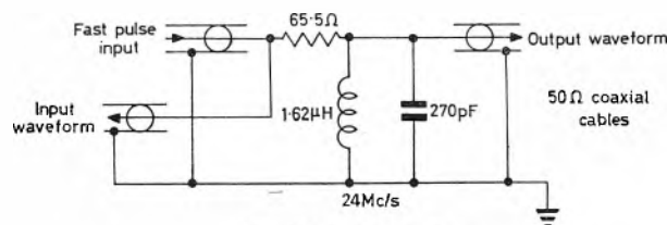
Fig. 12. Tuned circuit
