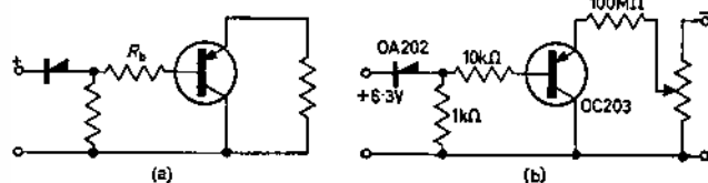
Fig. 2 (a). Switch inverted and diode added to prevent reverse bias at base (b). Measurement circuit to determine the 'off' properties of a silicon transistor
