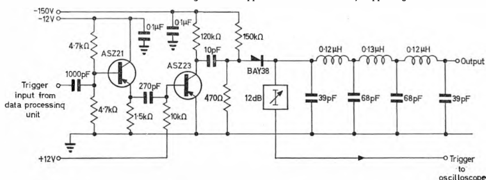
Fig. 5. Fast pulse generator and sampling filter
