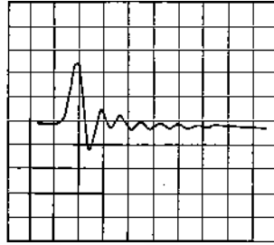
Fig. 6. Fast pulse generator output Y = 200\text{mV}/\text{div} X = 5\text{nsec}/\text{div}
