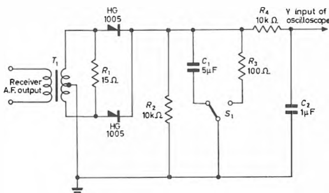
Fig. 4. Full-wave detector giving a voltage output proportional to the power dissipated in R_1 .
