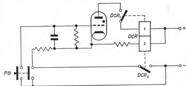
Fig. 7. Delayed switching with a thyatron
