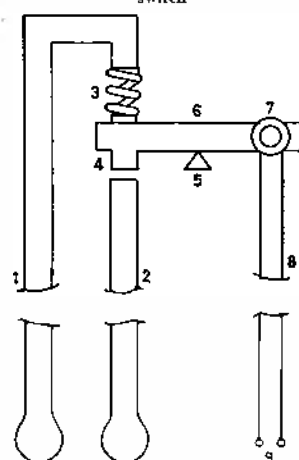
Fig. 11. Hotwire vacuum switch
