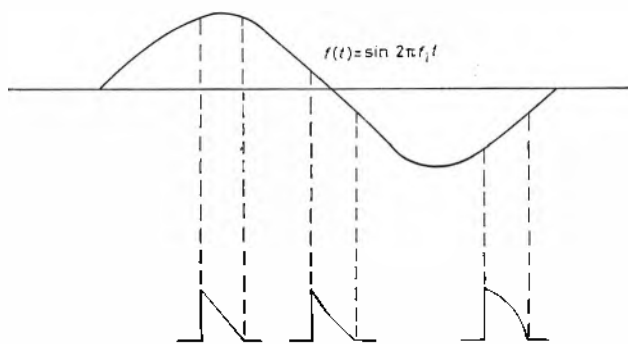
Fig. 3. Illustrating effects of large sampling times
