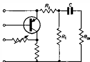
Fig. 6. Circuit giving reduced transient drift
