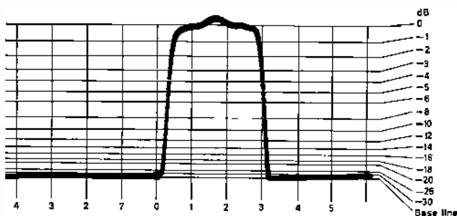
Fig. 2. Oscillogram of the frequency response characteristic of a single sideband receiver
