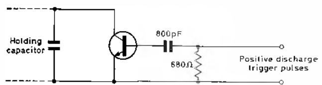
Fig. 7. Discharge circuit
