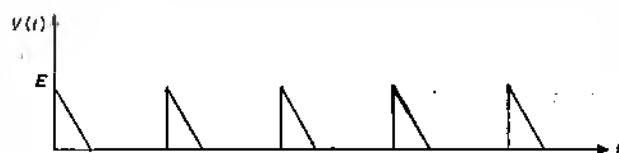
Fig. 2. Unmodulated triangularly shaped trailing edge pulses
