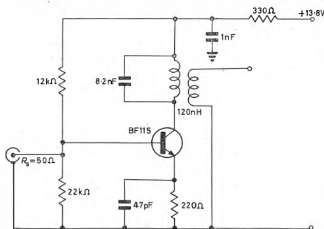
Fig. 9 Common-emitter amplifier
