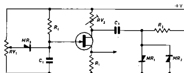
Fig. 3 Alternative method for controlling the period of oscillation
