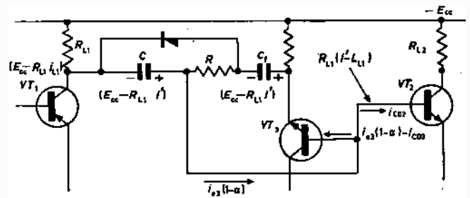
Fig. 5 Circuit to compute discharge-current capacitor C
