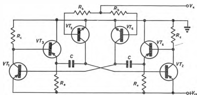
Fig. 5 Converter for wideband operation
