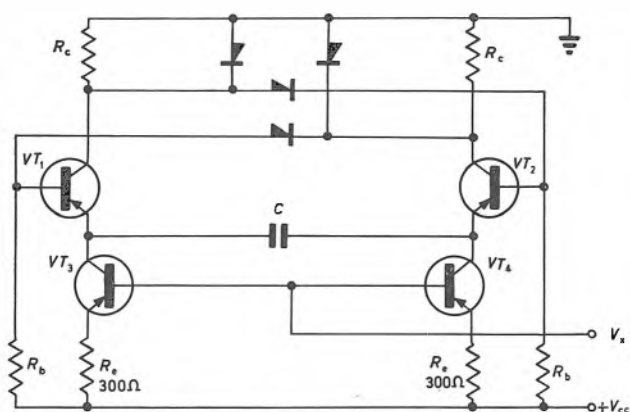
Fig. 4 Emitter-coupled multivibrator with constant-current sources
