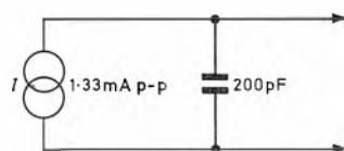
Fig. 10 Equivalent circuit of the delay-line output
