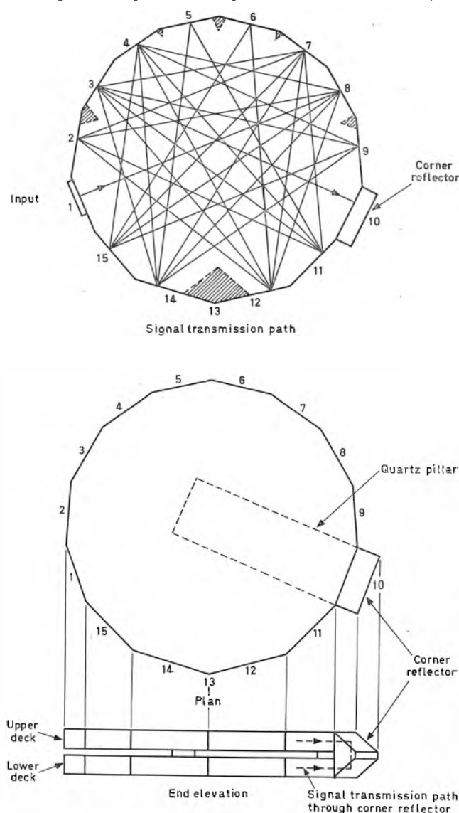
Fig. 1 Signal-transmission path and geometry of the 2.5ms delay line type-YL2104/09
