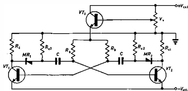
Fig. 6 Multivibrator with high input impedance
