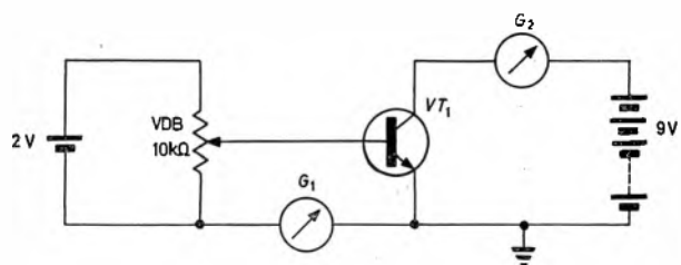
Fig. 6 Measurement of I_b , I_c and V_{be}
