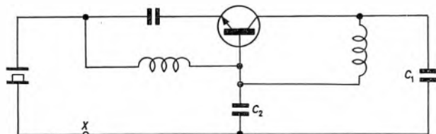
Fig. 3 Circuit of Fig. 2 redrawn with point X earthed
