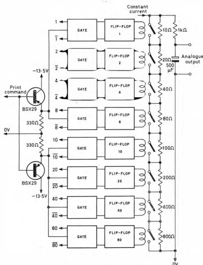
Fig. 1 General assembly
