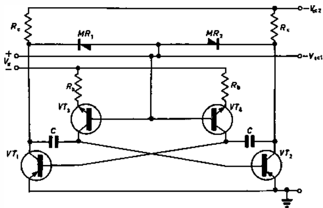
Fig. 3 Collector-coupled multivibrator with constant-current sources
