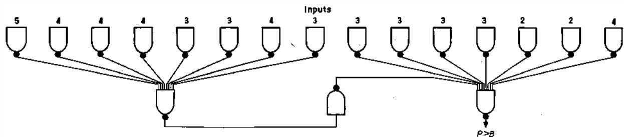
Fig. 9 Gates for comparison of preset decimal number P with binary-counter number B
