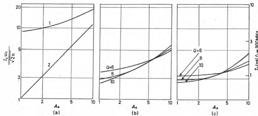
Fig. 5 Diagrams showing the normalized stage risetime T = T_{0\omega_i}/\sqrt{2\pi} and the actual stage risetime T_0 for when f_c = \omega_i/2\pi = 900\text{MHz} as a function of stage gain A_0 calculated for 2N976 transistors
