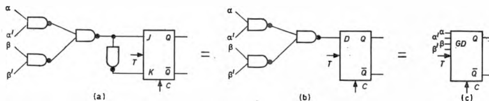
Fig. 7 (a) JK flipflop gated for bidirectional train counting (b) Equivalent D flipflop (c) Gated- D flipflop, where D = \alpha\alpha' + \beta\beta'
