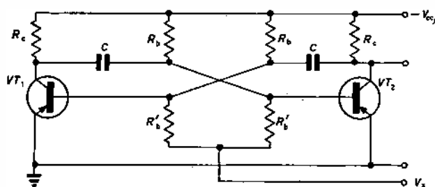
Fig. 2 Multivibrator with trimming frequency-adjustment voltage V_x
