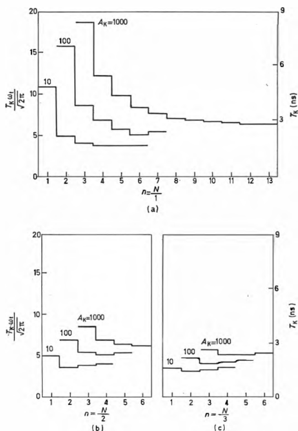
Fig. 7 Normalized n -stage cascade risetime T_K\omega_i/\sqrt{2\pi} as a function of the number of stages n and for several values of cascade gain A_K , for
