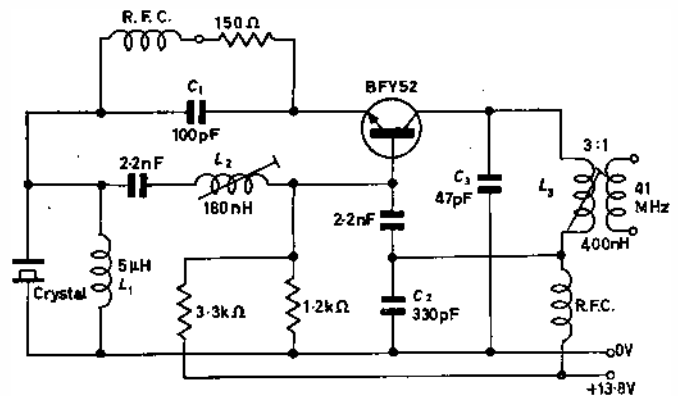
Fig. 6 Complete circuit
