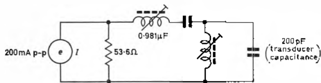
Fig. 8 Bandpass equalizing network modified to suit a constant-current source
