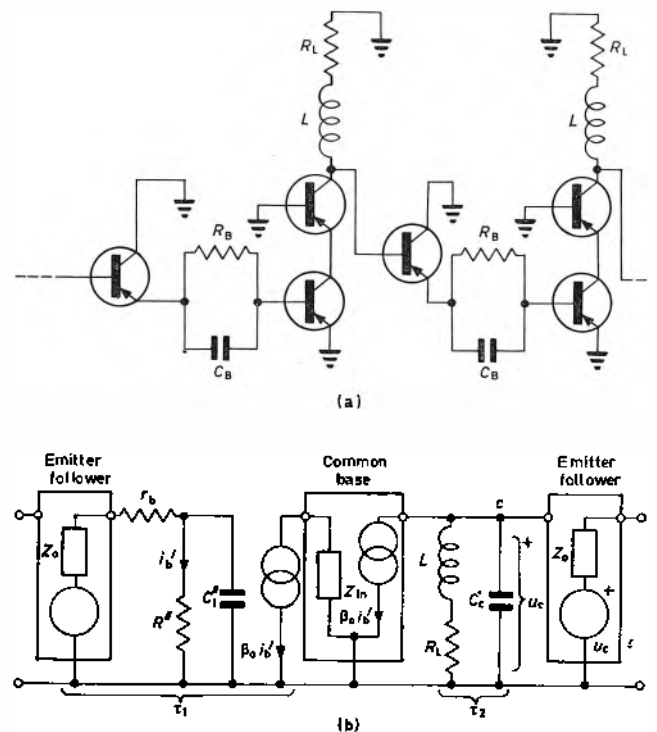
Fig. 4 (a) Cascode circuit with both collector and base compensation and with an emitter follower as an interstage when connected in a cascade. (b) Equivalent circuit
