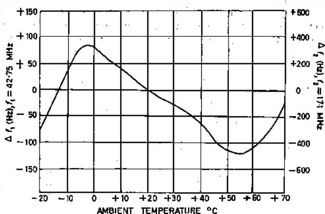
Fig. 8 Variation of output frequency with temperature
