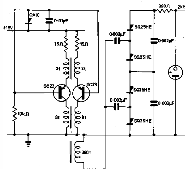
Fig. 6 Circuit for 2kV fixed, 1mA stabilized
