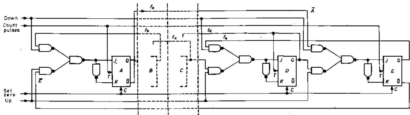
Fig. 5 Bidirectional train counter
