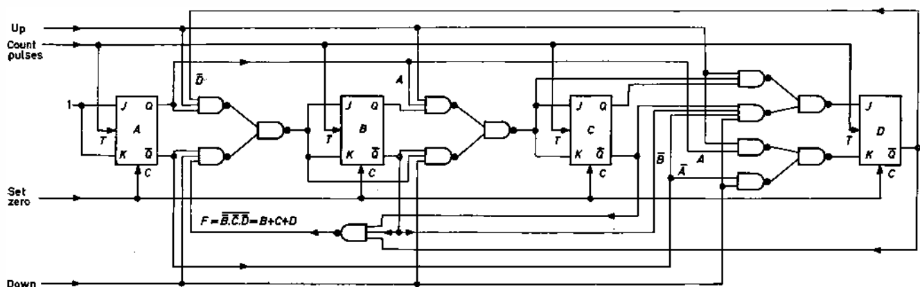
Fig. 6 Bidirectional binary decade counter
