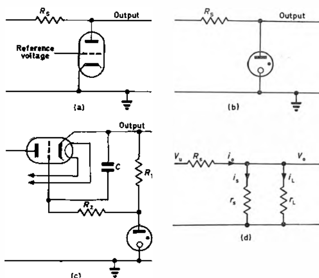
Fig. 2 Shunt stabilization
