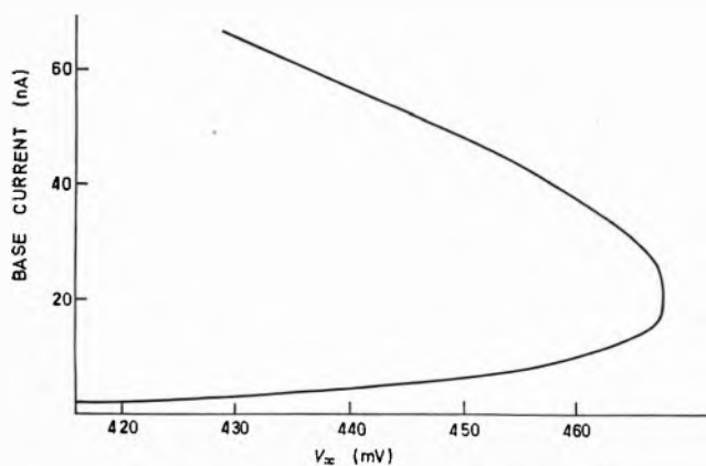
Fig. 8 Experimental curve of V_x versus I_b
