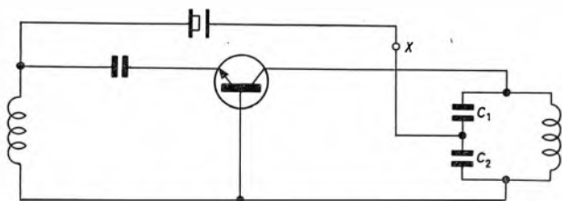
Fig. 2 Circuit of Fig. 1 with impedance-transforming network
