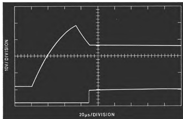
Fig. 7 Oscilloscope traces (redrawn) when the voltage of a pulse is locked at an instant of decreasing value
