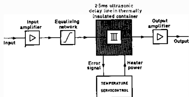
Fig. 3 Block diagram of the 2.5ms delay unit
