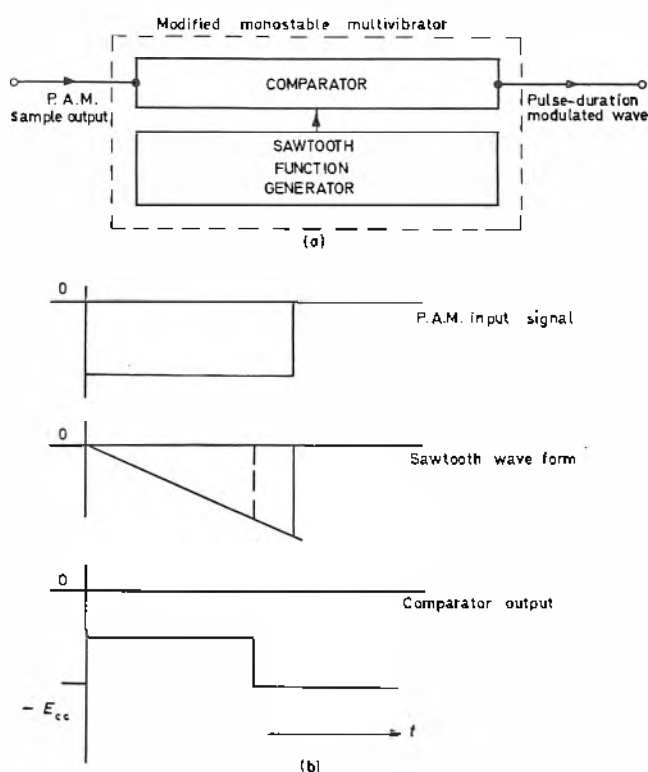
Fig. 2 Method of p.a.m./p.d.m. conversion (a) Block diagram (b) Waveforms
