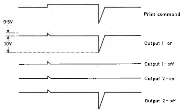
Fig. 4 Gate-output signals
