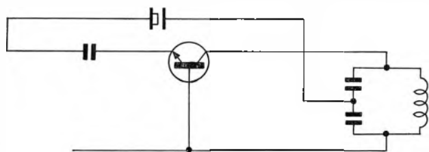
Fig. 1 Basic configuration
