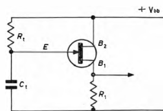
Fig. 1 Common unijunction-transistor astable circuit
