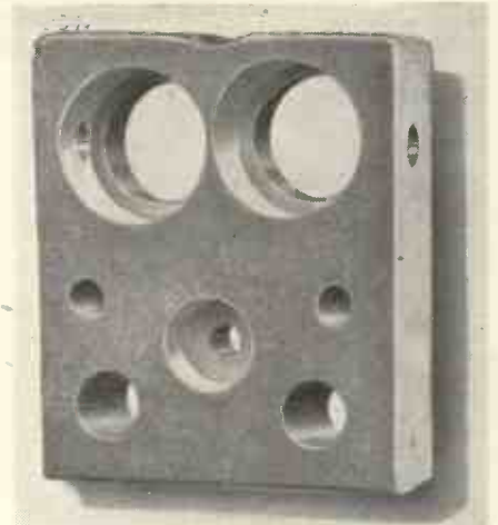
Fig. 6. A slab of Mycalex showing the variety of holes which can be drilled without chipping of the surface.
