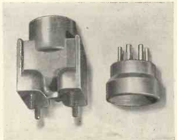
Fig. 8. Mycalex moulded lamp socket and valve base.
