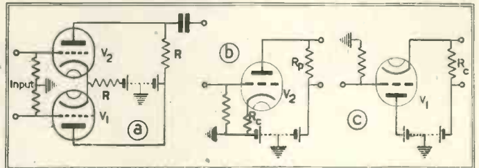
Fig. 6. Tönnies' differential input circuit and its equivalents.
