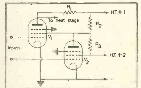
Fig. 4. Schmitt's differential amplifier using high gain pentodes.
