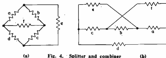
Fig. 4. Splitter and combiner
