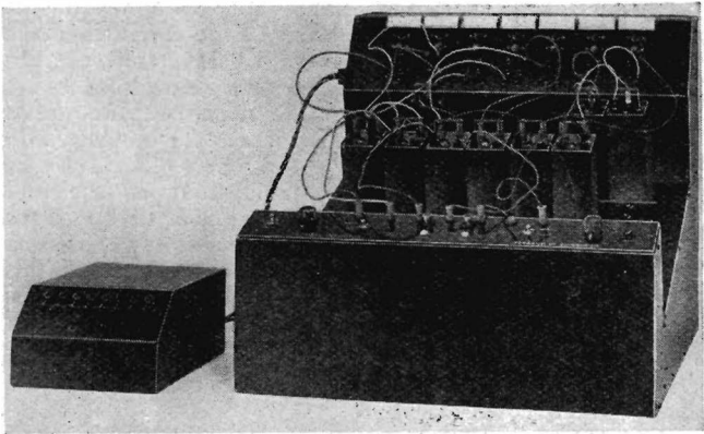
Fig. 7. View of Computer set up for Problem III Leads come from the variables to the connective boxes and from the outputs of the connective boxes to the sockets in the control panel, the latter sockets being the inputs of the "AND" box which detects answers.
