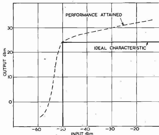
Fig. 3. Microphone amplifier input-output characteristics
