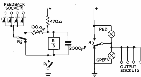
Fig. 8. (Above). Circuit diagram of sensitive variable unit
