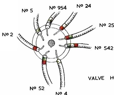
Examples of colour coded wires and cableforms
