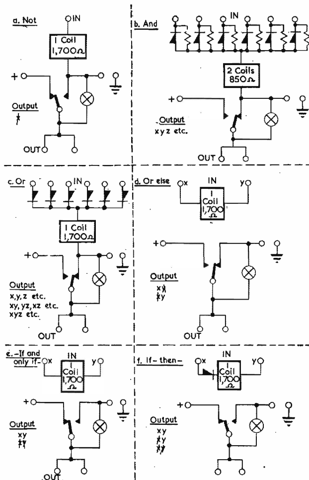
Fig. 2. Connective boxes for the Logical Computer
