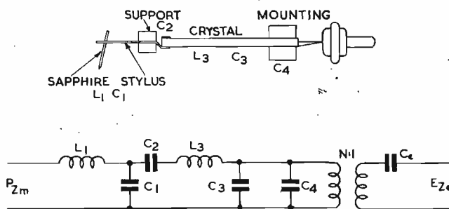
Fig. 10. Mechanical and electrical constants of high fidelity gramophone pick-up
