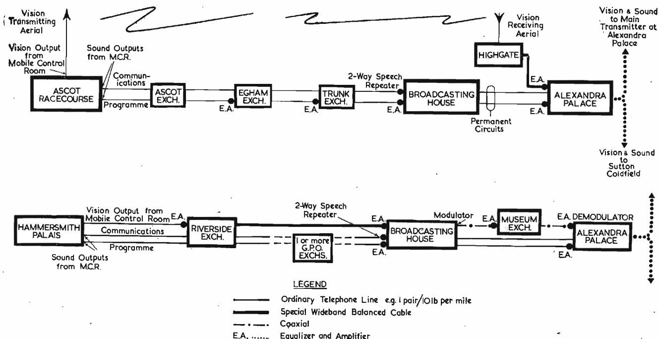
Fig. 8. Schematics of typical O.B. links. (a) Vision by radio, sound by cable. (b) Vision by cable, sound by cable
