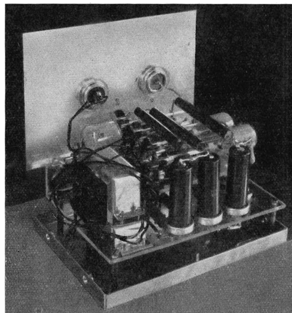
Fig. 4. A corona stabilizer power supply unit
