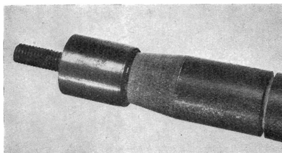
High strength and durability are features of 'Araldite'. Here, Type 1 adhesive is used to bond metallic ferrules to Mycalex insulator rods for high-voltage apparatus.
