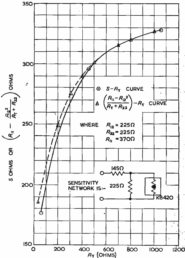
Fig. 9. Matching of R'-R T and S-R T curves to give a useful degree of temperature compensation
