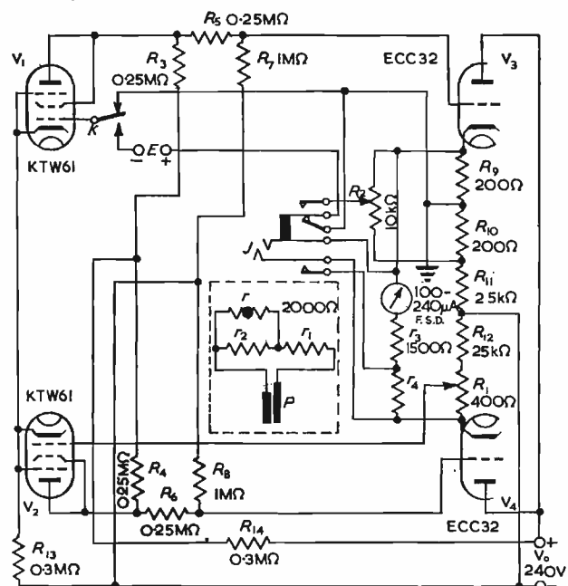
Fig. 5. A practical circuit using KTW61 valves
