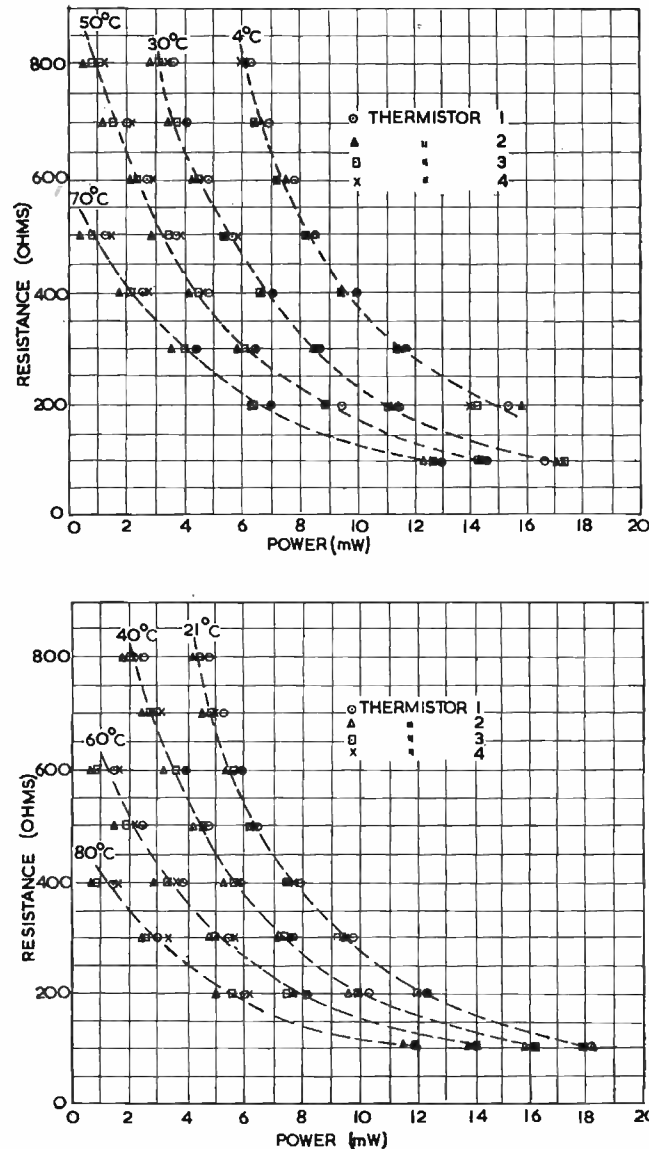
Figs. 2 (a) and (b). Resistance-power curves for bead thermistors type E2361/20
