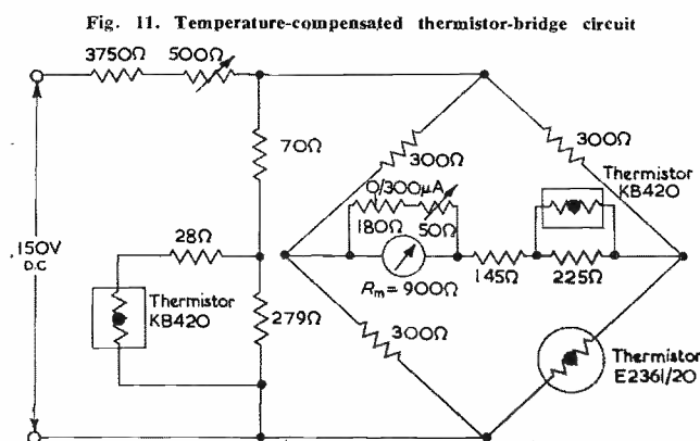
Fig. 11. Temperature-compensated thermistor-bridge circuit
