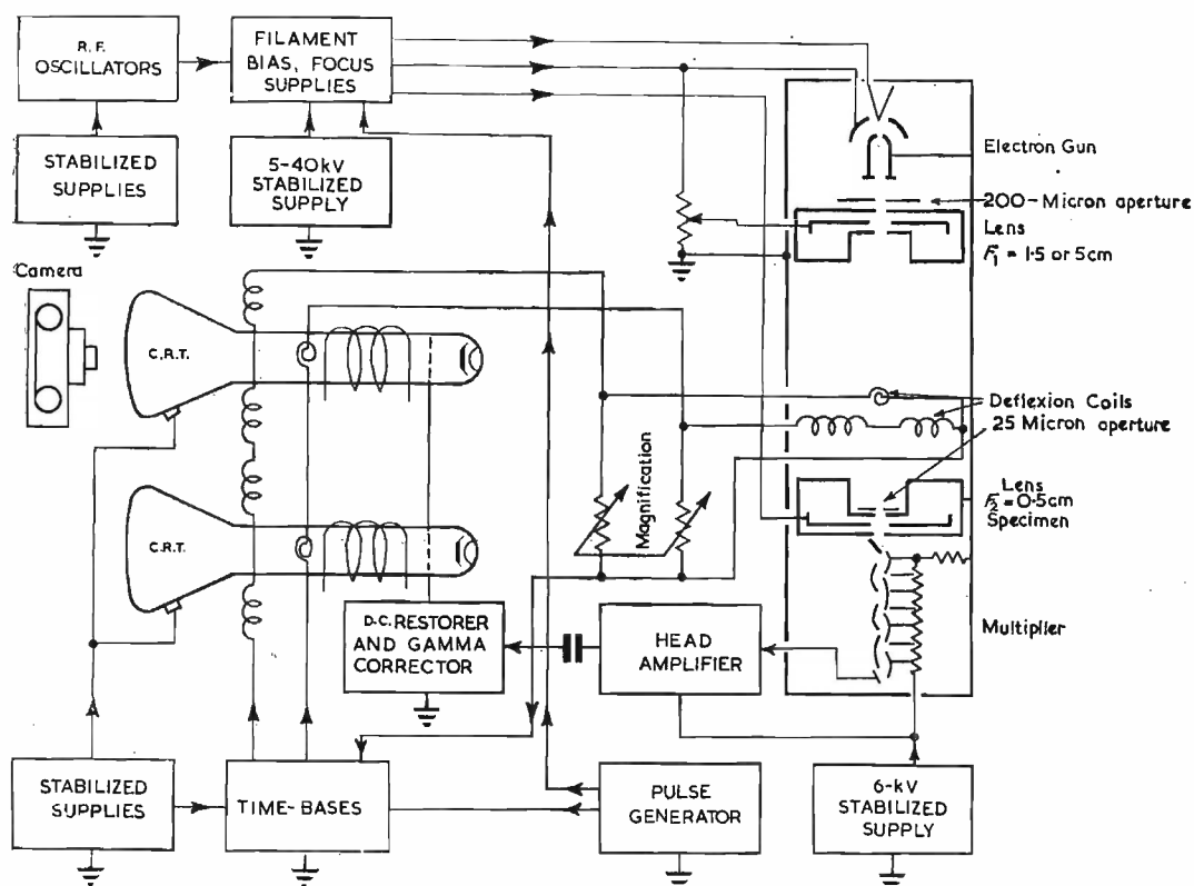
Fig. 2. Block schematic diagram of scanning electron microscope
