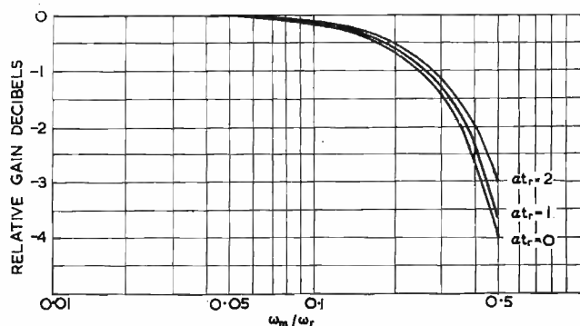
Fig. 14. Attenuation distortion characteristics of pulse lengtheners
