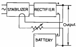
Fig. 5. Boost operation.
