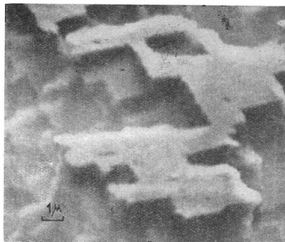
Fig. 7. Etched aluminium. Angle 25°, magnification ×6000, 16kV, 10^{-12} A beam current, exposure 300 seconds
