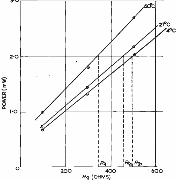
Fig. 7. Power/meter-arm resistance curves for bridge circuit
