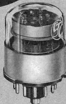
GI0/241E "Nomotron" Unidirectional Cold- Cathode Gas Tube Decade Counter
