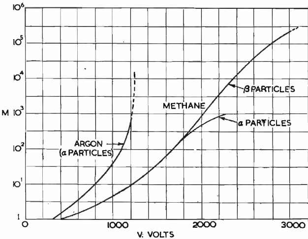
Fig. 1. Gas Multiplication (M) / Anode Voltage (V) Flow counter. Argon and Methane, atmospheric pressure brass cathode 35 mm. dia., anode wire 0.012 mm. dia.
