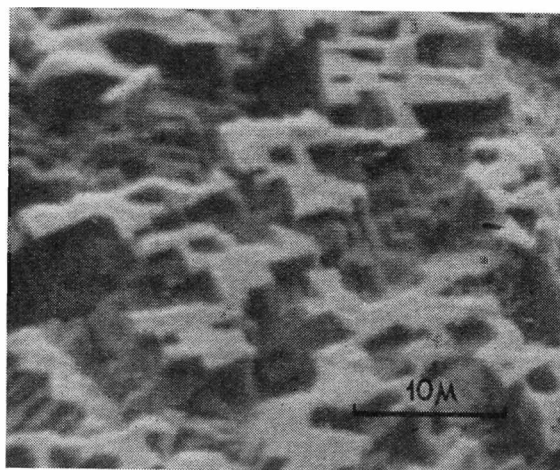
Fig. 6. Etched aluminium. Angle 25°, magnification ×2000, 16kV, 1.5 \times 10^{-10} A beam current, exposure 5 seconds
