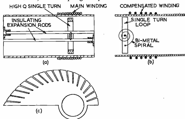
Fig. 1(a). Sectionalized view of inductive temperature compensator Fig. 1(b). Inductive compensator with single turn loop free to move on spindle to which bi-metal spiral is anchored.
