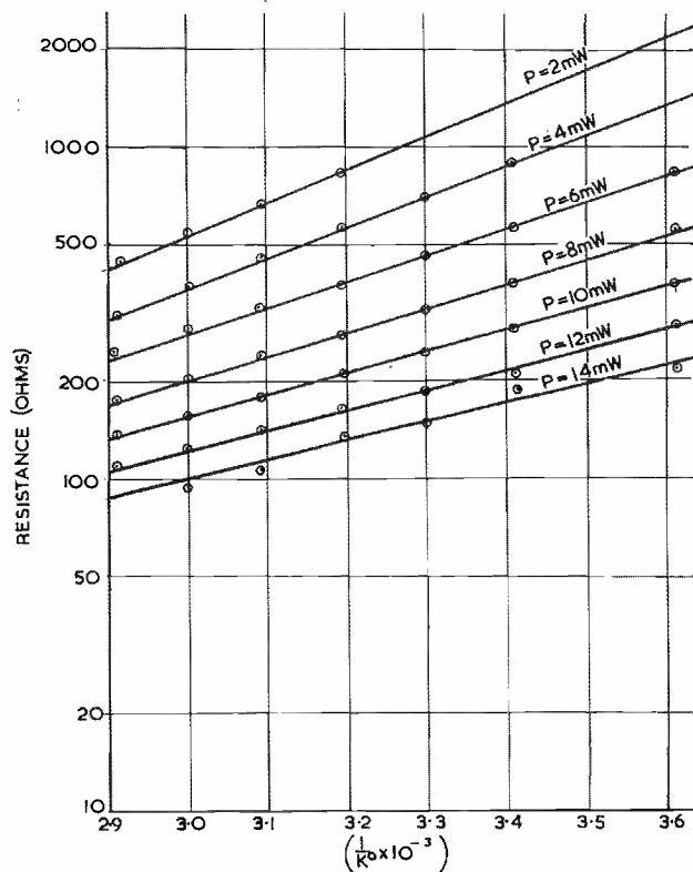
Fig. 12. Characteristics of bead thermistors type E2361/20
