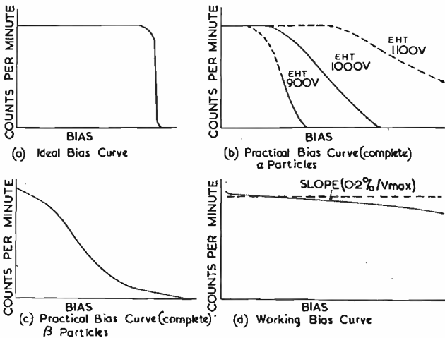
Fig. 2. Bias curves
