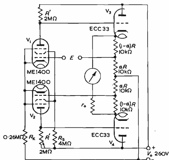
Fig. 4. A practical circuit
