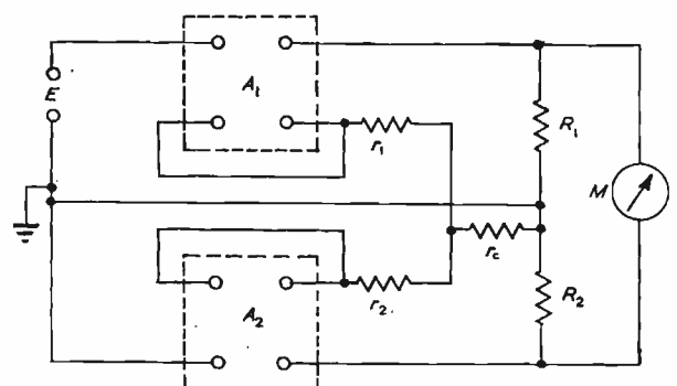
Fig. 2. Modification using common feedback resistor
