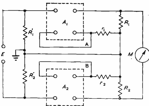
Fig. 1. Simple form of differential amplifier
