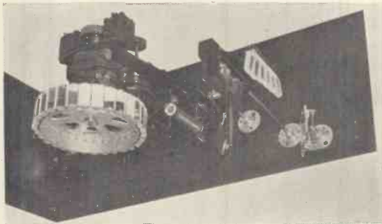
Fig. 3.—This photograph shows the assembly of the mirror-drum receiver including the ray divider or vertical scanning.
