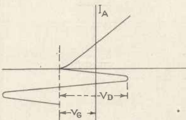
Fig. 2.—Here is the I_a/V_g characteristics of a final P.A. stage biases to cut off.
