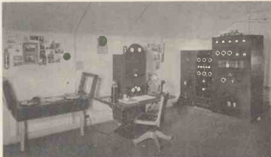
From left to right will be seen recording gear, electric gram-motor and pick-up, radio receiver, mixing panel, cathode-tube monitor and ribbon microphone, and finally the all-wave band transmitter and class B modulator.
