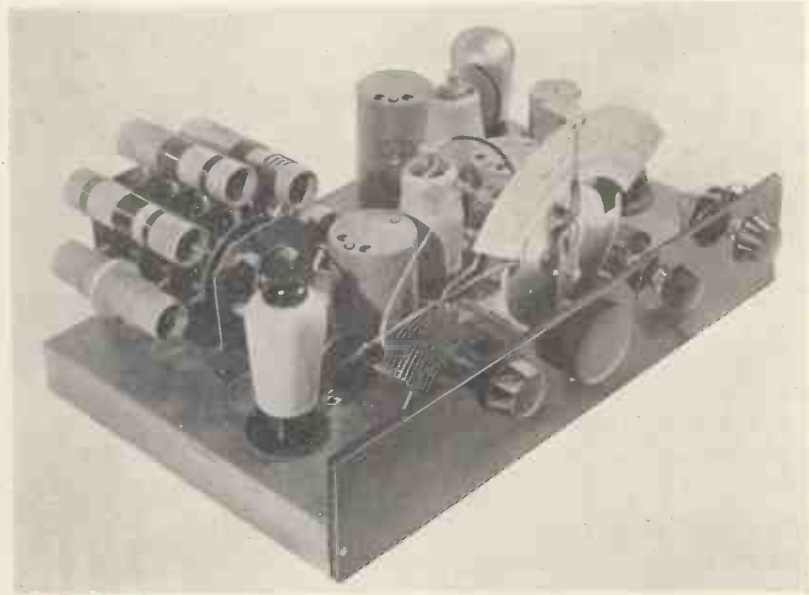
Here is the receiver chassis. The panel is only a temporary one used to secure the tuning components during testing.
