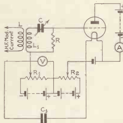
This is the circuit for the suggested meter. It is better to use this than to rely on the fact that 23 per cent. rise should mean 100 per cent. modulation.
