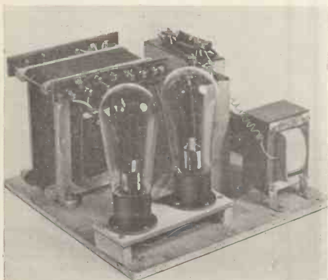
Photograph of the power unit for 7-metre transmitter.
