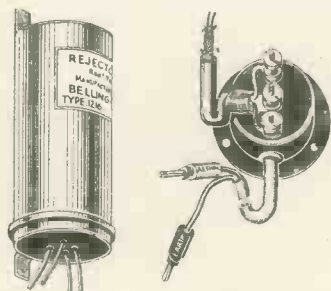
On the left is the first impedance matching transformer connected close to the aerial at the top of the mast. The second transformer is fitted to the receiver chassis.
