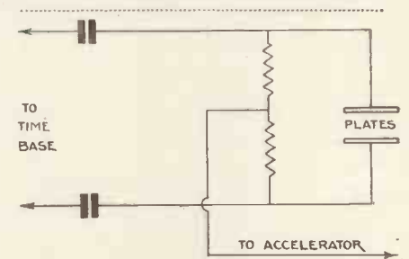
Fig. 5.—Symmetrical circuit for balancing potentials applied to the deflector plates to overcome distortion.
