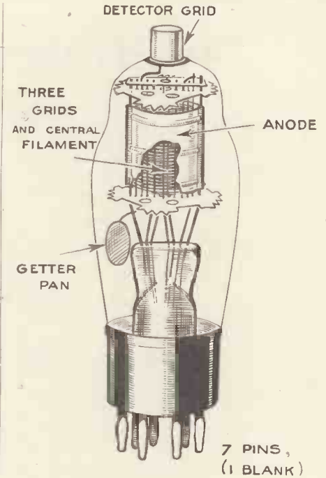
Fig. 5.—All the electrodes in this Osram heptode can be quite clearly seen. A point to remember is that the control grid is taken to the top cap.
