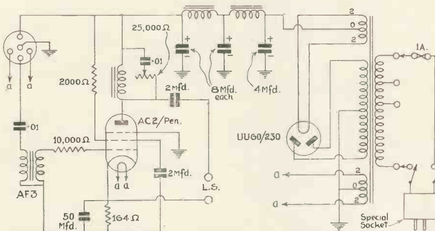
This section of the circuit is entirely self-contained. It gives 3,400 milliwatts output with only a moderate input. The power pack gives 250 volts H.T. at 60 milliamperes.
