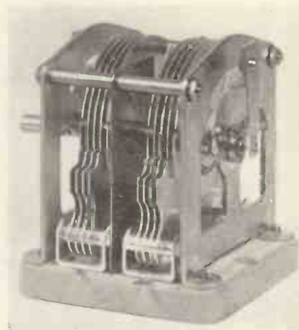
The Radiomart two-gang split stator variable condenser.
