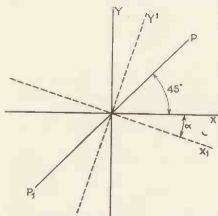
Fig. 2.—The circular polariser and analyser.—PP 1 is the nicol with quarter-wave plate OX; OX 1 is the analysing quarter-wave plate.
