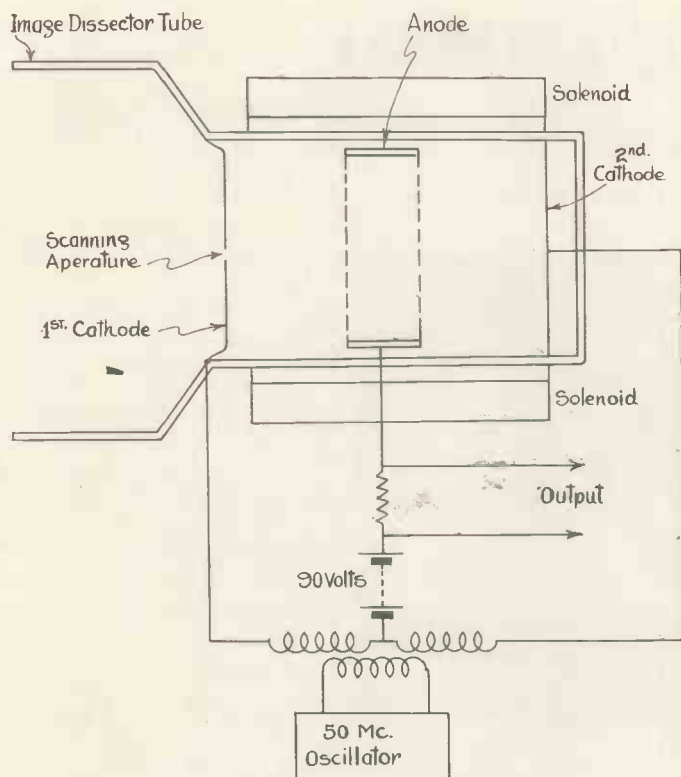
Fig. 2.—Electron multiplier for use with image dissector tube.
