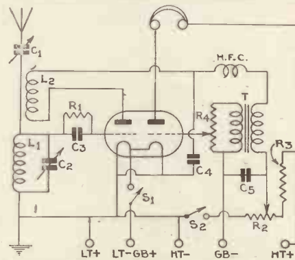
(Right)—A B21 is the type of valve used in this two-in-one circuit. Even though it is novel, the results given are good. It is a fine receiver for the beginner on short waves.
