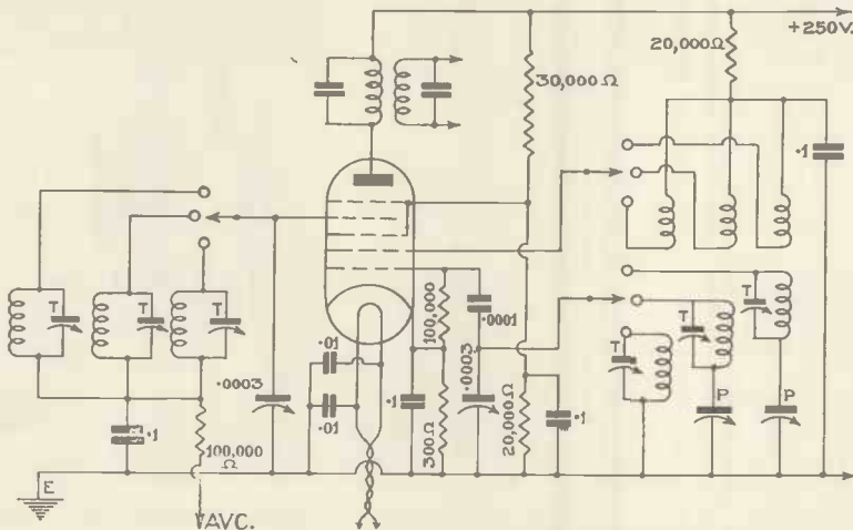
Fig. 1.—This is the heart of an efficient short-wave super-het. It can be added to almost any short-wave super but preferably one with 450 kc. I.F. transformers.
