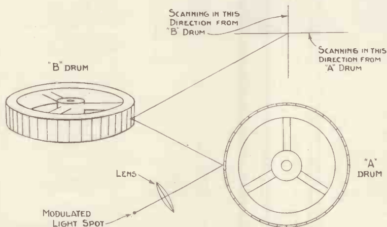
A suggested scheme for high-definition mechanical scanning employing two mirror-drums.
