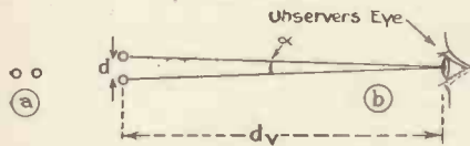
Figs. 1a and 1b Diagrams illustrating the optimum viewing distance.
