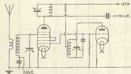
Fig. 3.—For ultra short-wave and/or television reception a separate oscillator is recommended in this circuit.
