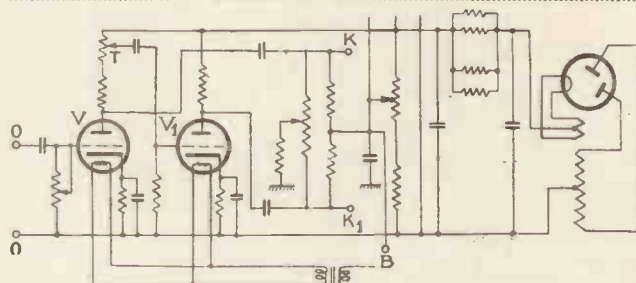
Circuit of push-pull system for cathode-ray tube.
