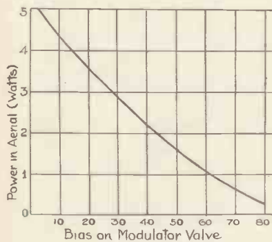
Fig. 6 (left).—Modulation characteristic.
