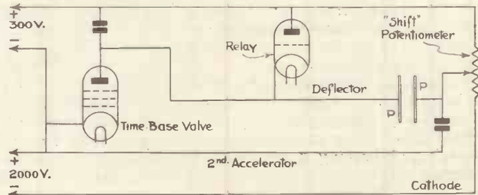
Fig. 3.—Showing how the deflector plates P differ appreciably in potential from the second accelerator. This causes de-focusing of the beam on parts of the screen.
