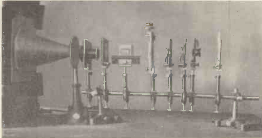
A photograph of the circular polariscope in use.
