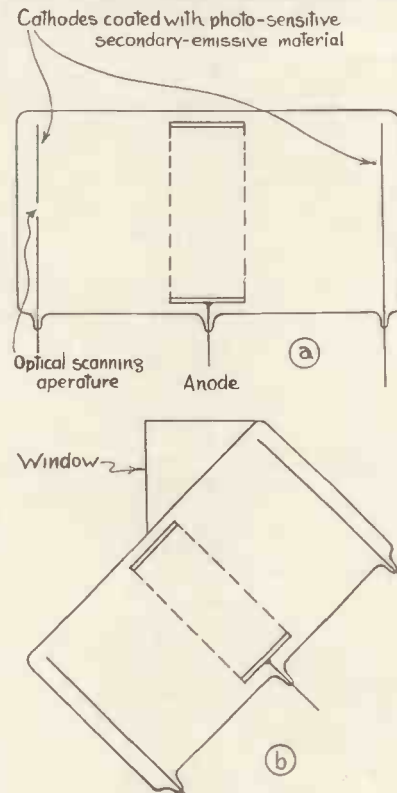
Fig. 3.—Secondary emission photo cells (a) for use with mirror-drum transmitter, (b) for use with disc receiver.
