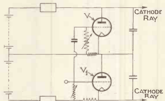
Fig. 1.—Circuit for producing interleaved scanning. Patent No. 423,101.
