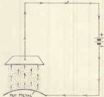
Fig. 2.—Electrons being collected by a metal plate connected to the positive terminal of a battery.
