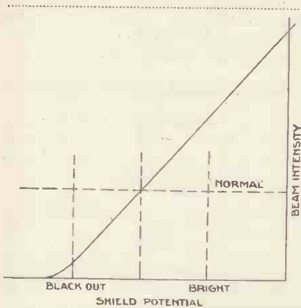
Fig. 1.—Ideal curve of beam intensity—shield potential giving full modulation with no distortion.
