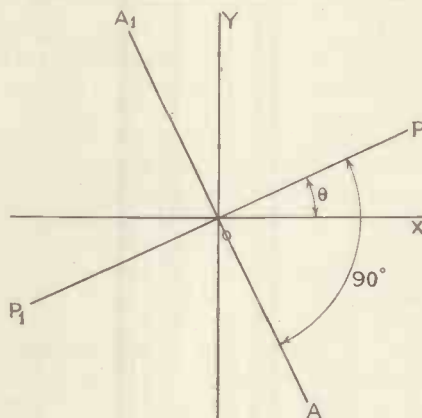
Fig. 1.—Linear polariscope with crossed nicols.— PP' is the vibration direction of polariser; AA' is the vibration direction of analyser; OX, OY are the vibration directions of birefringent section in the polariscope.
