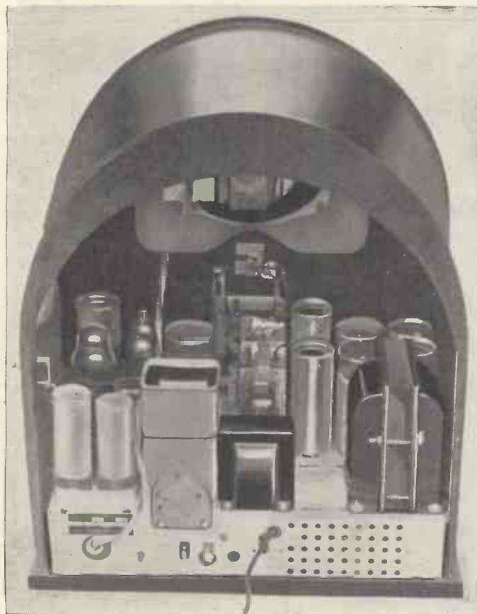
This all-wave receiver although it uses eleven valves is no larger than the average broadcast super-het. Ganged tuning, single dial control and A.V.C. on all wavelengths are only three of the many features of this receiver. Five tuning scales, all calibrated in frequencies, is a fine idea for it overcomes the difficulty of designing a clear tuning scale.
