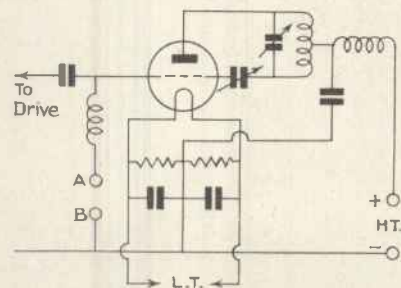
Fig. 4.—With this circuit in use the P.A. will operate down to 10 metres with grid modulation.
