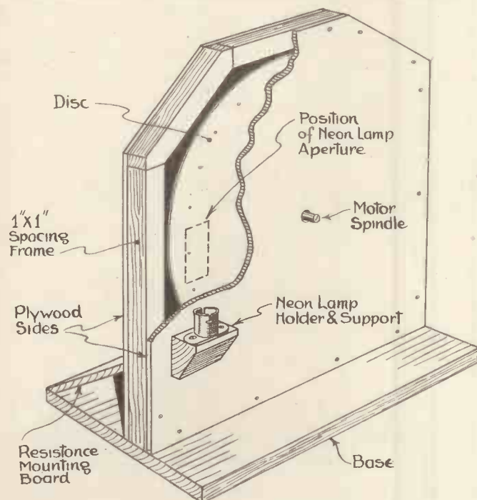
A cut-away sketch showing the essential parts of the viewer.
