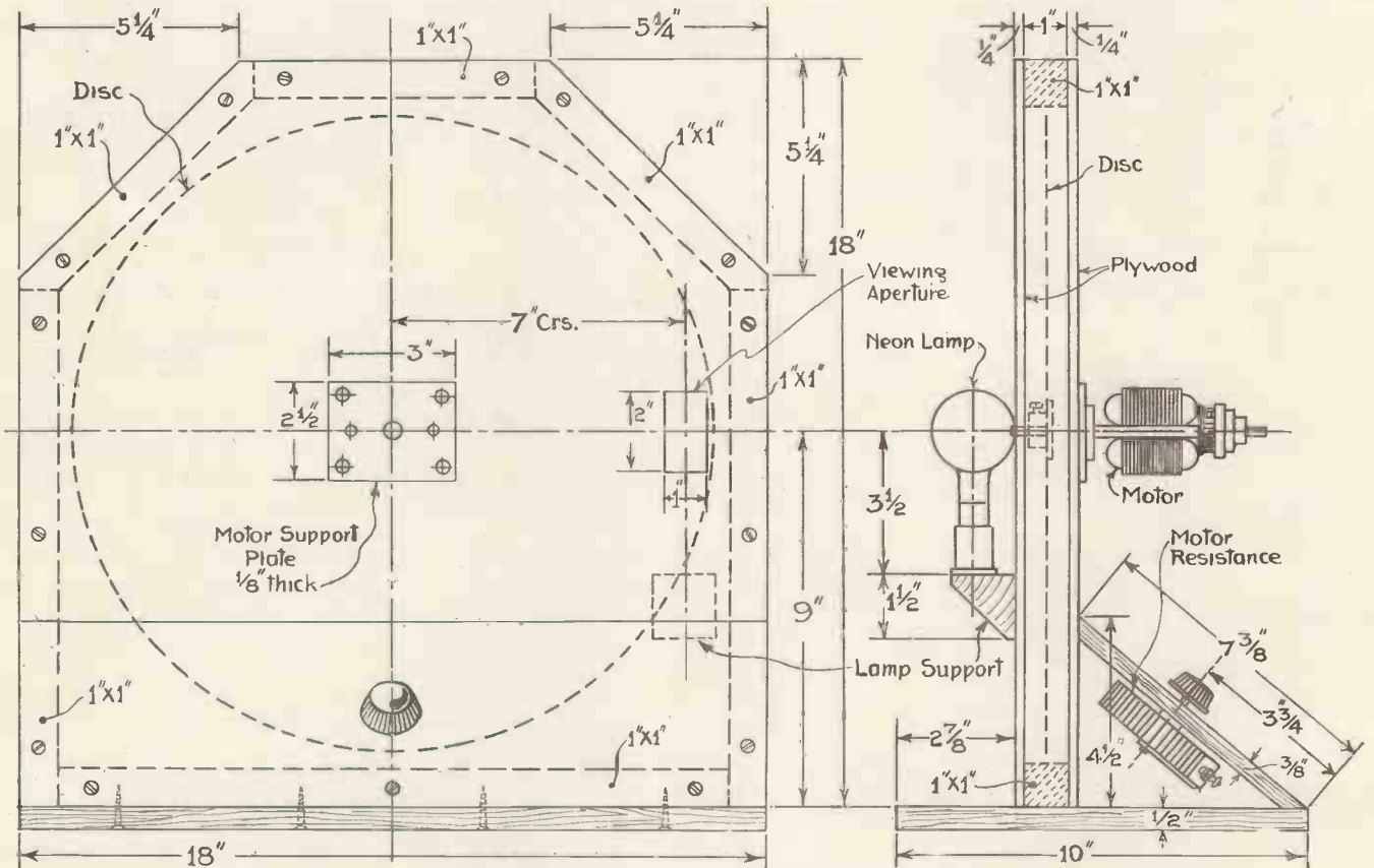
Fully dimensioned drawings of front and end elevations of the receiver. All the necessary constructional details are quite clear.
