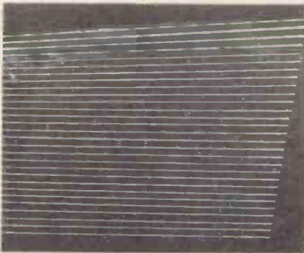
Fig. 4.—A line screen in the form of a trapezium caused by interaction of the deflector plates with high scanning potentials.
