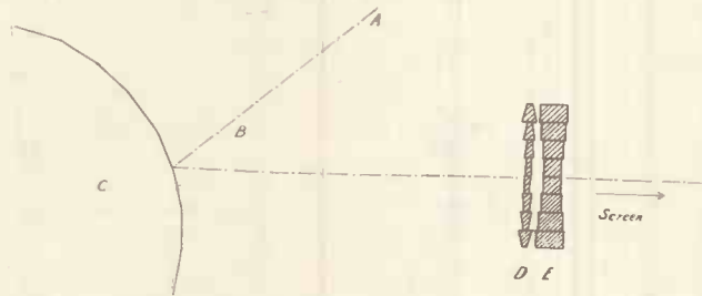
Fig. 1.—A plan view showing the relative positions of ray divider and mirror-drum for horizontal scanning.
