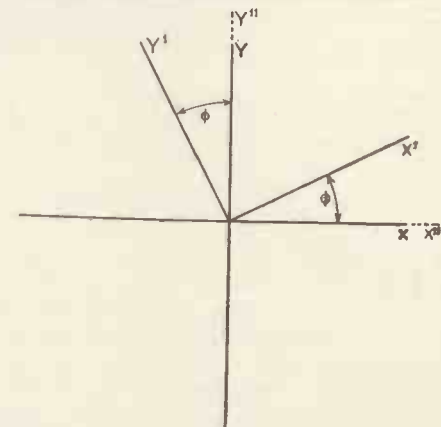
Fig. 3.—OX=fast direction of first quarter-wave plate; OX' =fast direction of birefringent section; OX''=fast direction of analysing quarter-wave plate.
