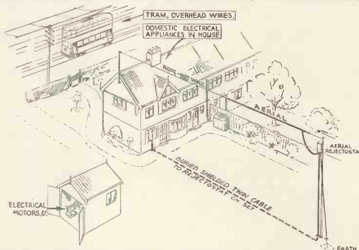
Where the interference is local it is advisable to bury the lead-in wires as much as possible. This is particularly advisable when the interference is from car ignition or small motors.
