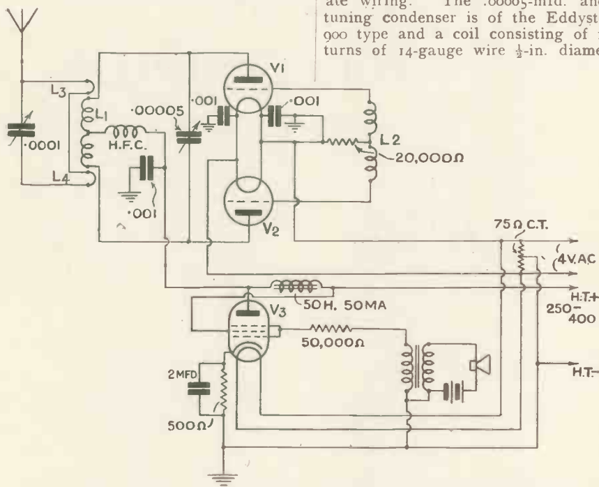
This modulated five-metre transmitter is very stable in operation. The 200 miles record set up last year used a fundamentally similar circuit.
