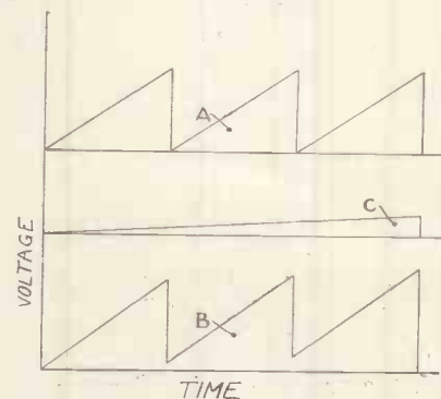
Fig. 2.—Wave-forms for interleaved scanning. Patent No. 423,101.
