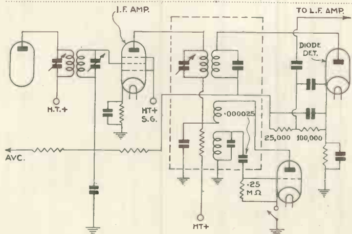
Fig. 2.—In this arrangement it is important that the beat note oscillator be tuned to a harmonic of the C.W. station and not to the fundamental. By introducing the oscillator signal into the diode circuit no complications are set up when automatic-volume-control is applied to the I.F. or H.F. stages.
