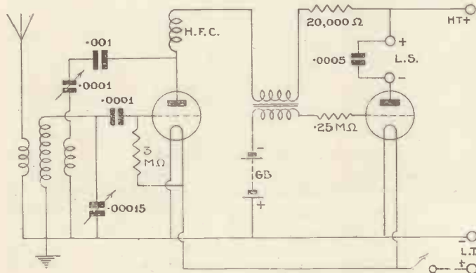
Here is the circuit for the Beginner's Two. There is only one high-tension voltage tapping; it is impossible to short-circuit high-tension to the reaction condenser owing to the use of a series blocking condenser.
