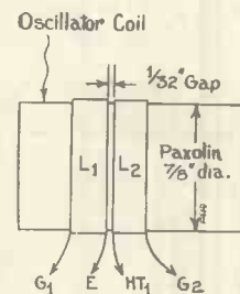
Fig. 4.—Here is the coil former, all the necessary winding data are given in the text in concise form.
