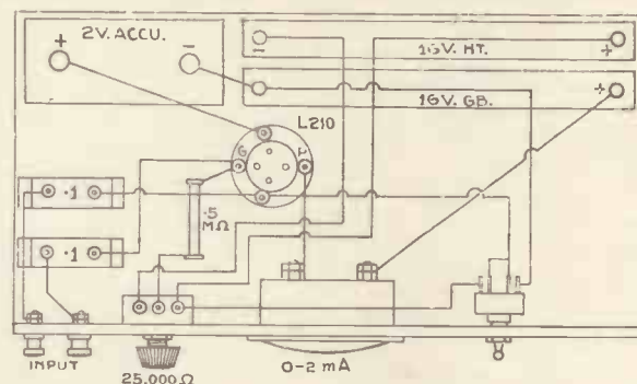
This is the suggested lay-out for the components which can be modified if desired.
