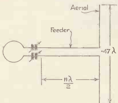
Fig. 5 (right).—Theoretical circuit of transmitter.
