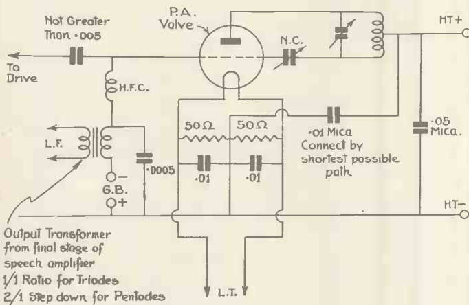
Fig. 1.—This is a typical P.A. circuit in a driven transmitter.
