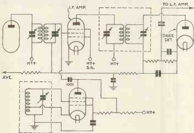
Fig. 1.—By feeding the output from a beat note oscillator into the grid of an I.F. amplifier, C.W. reception is considerably simplified. No super-het receiver without an oscillator of this kind is suitable for C.W. reception.
