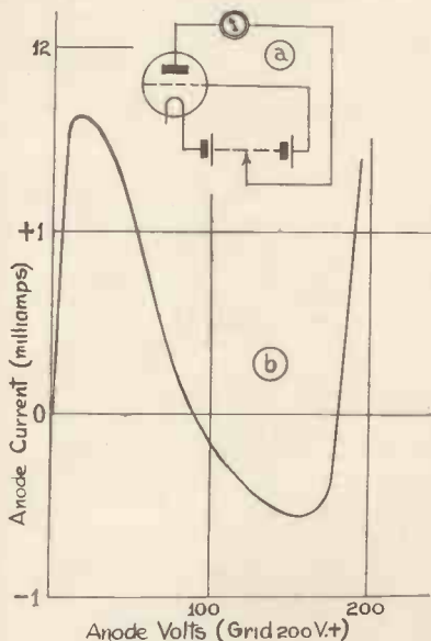
Fig. 1.—(a) Circuit to show secondary emission. (b) Anode current curve for triode with coated anode.
