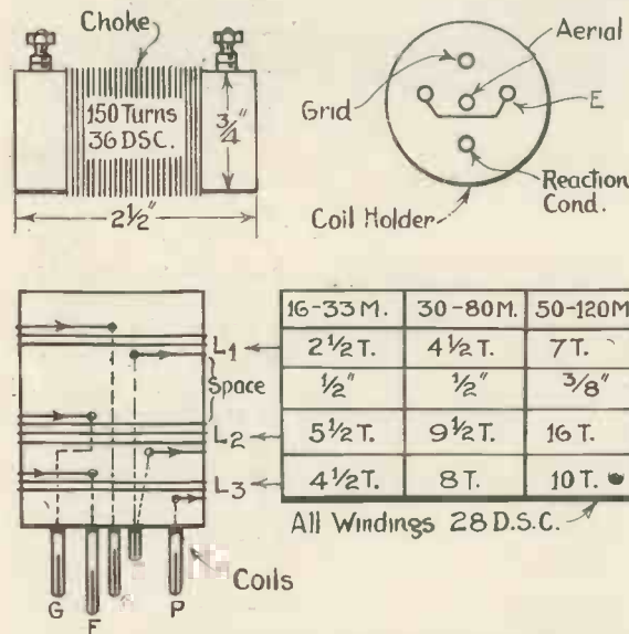
All the necessary details for winding the coils for the Beginner's Two and other simple receivers are given above.
