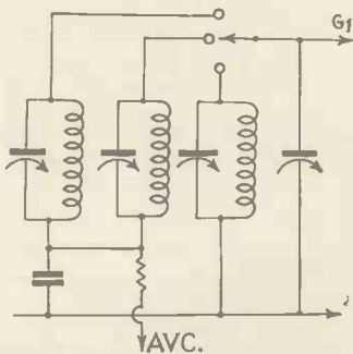
Fig. 2.—It is suggested that on the 25-megacycle band automatic-volume control be omitted. Notice that the third coil is then connected to earth.
