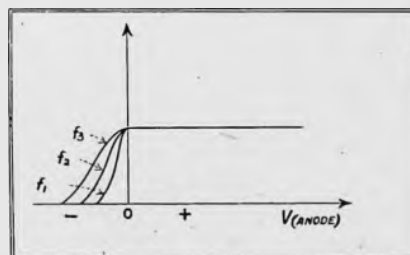
Fig. 2—Effect of varying wavelength, with constant intensity.
