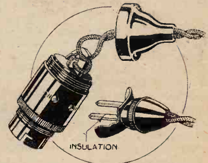
"Xtra-Point" lamp holder. It is shrouded in bakelite and fitted with two-pin plug for extension lead. Can be used to supply a battery eliminator.
