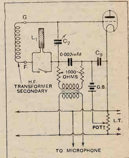
How to introduce a microphone into the detector circuit of the "Everyman Four."
