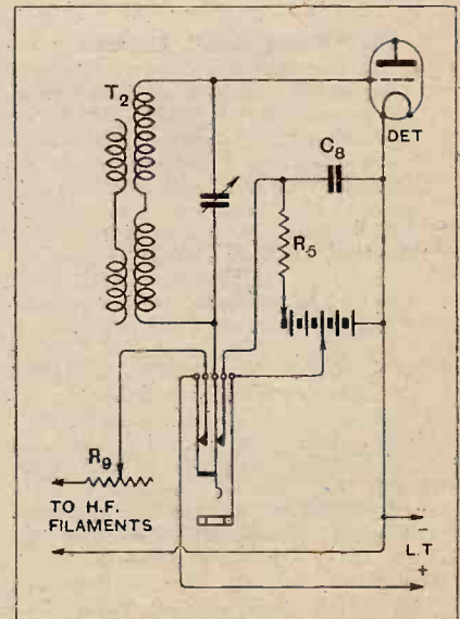
Fig. 1.—A pick-up jack arranged for automatic control of H.F. filament circuits.
