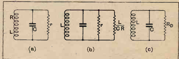
Fig. 2.—(a) Shunted tuned circuit. (b) and (c) Equivalent circuits. R_D is the resultant dynamic resistance and is given by \frac{I}{R_D} = \frac{I}{r} + \frac{CR}{L} .
