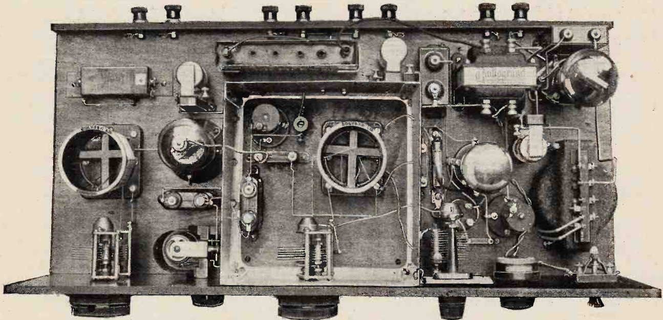
Plan view of receiver showing the straightforward layout of the H.F. stage.
