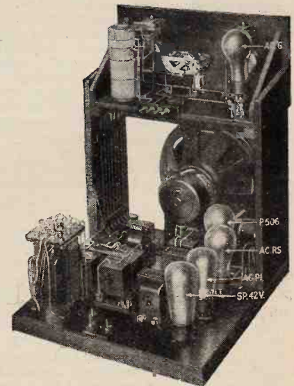
Amplifier-receiver unit for A.C. mains. The receiver unit and control panel are mounted above the loud speaker, while the power amplifier and rectifier units occupy the base platform.
