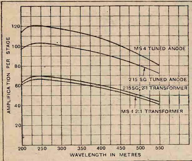
Fig. 5.—Amplification per stage with 2in. coil, as tuned anode coil and as secondary of 2:1 step-up transformer.
