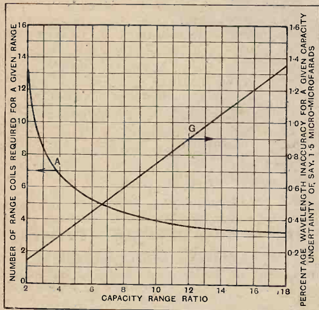
Fig. 2.—Curves showing the number of range coils and capacity ratio of condenser of a wavemeter.
