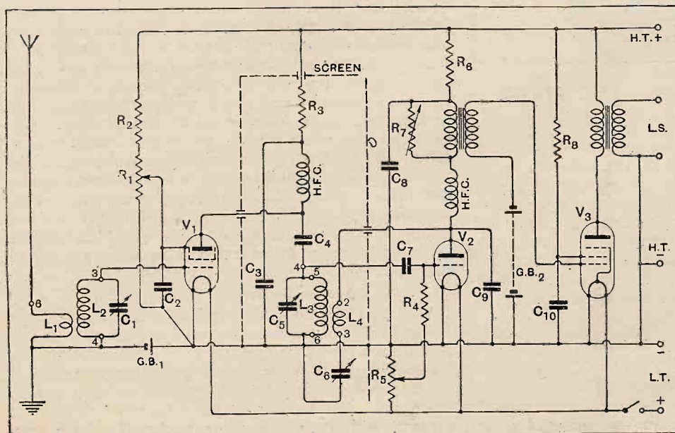
Fig. 1.—The theoretical circuit values are as follows: C_1 and C_5 = 0.00015 mfd., C_2 and C_3 = 0.01 mfd., C_4 and C_9 = 0.0002 mfd., C_6 = 0.0001 mfd., C_7 = 0.000075 mfd., C_8 = 2 mfd., C_{10} = 1 mfd., R_1 = 30,000 ohms, R_2, R_3 and R_5 = 20,000 ohms, R_4 = 5 megohms, R_5 = Polar semi-fixed potentiometer, R_7 = 200,000 ohms, R_8 = 5,000 ohms.
